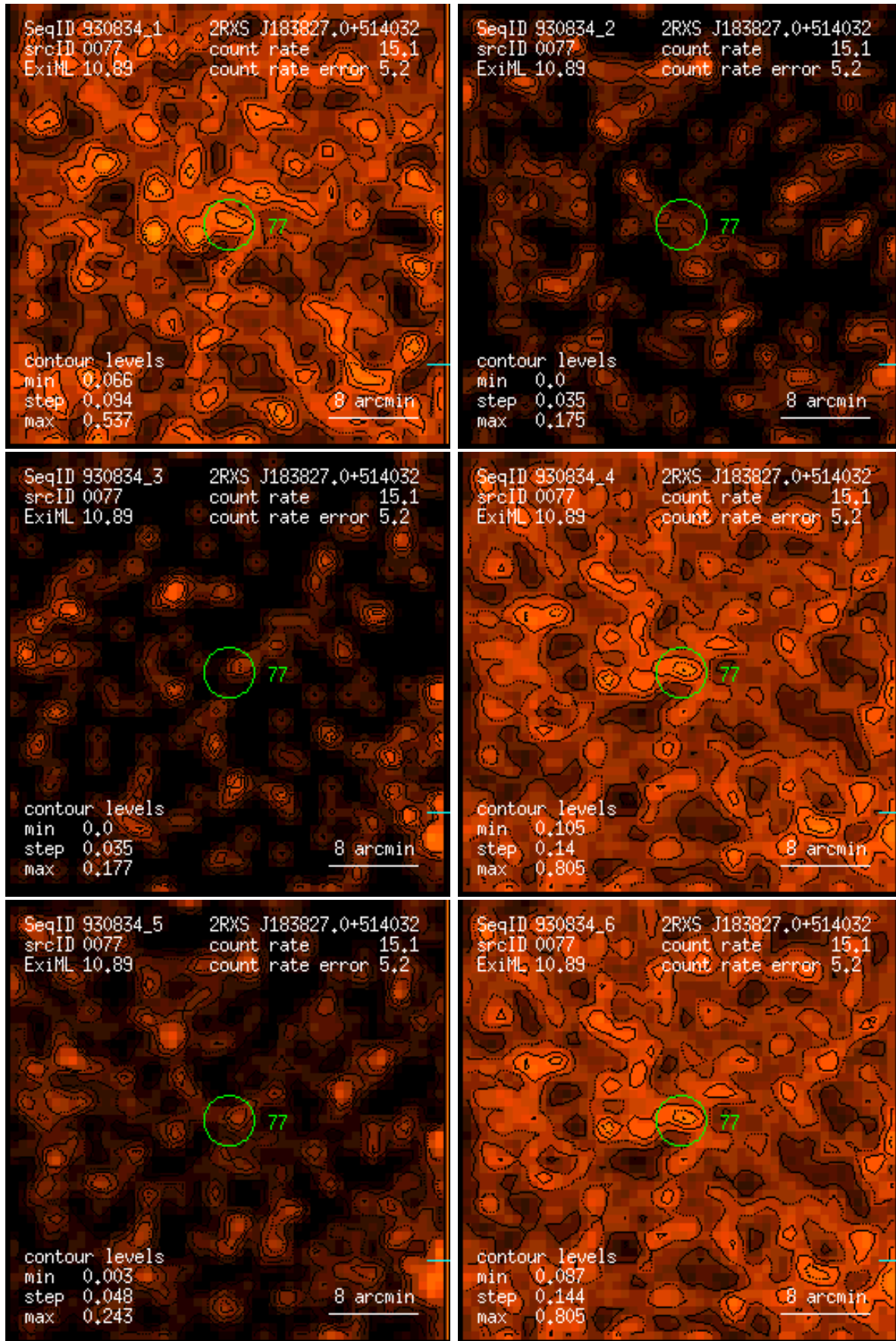
Figure 77: RASS 930834: detection 0077: band rate images, Gaussian filter: (1) PSPC channels 11 – 41, (2) 52 – 90, (3) 91 – 201, (4) 11 – 235, (5) 52 – 201, (6) 11 – 201. Broad band rates in counts/ks. Band rate contour levels in counts/ks/arcmin 2 .
