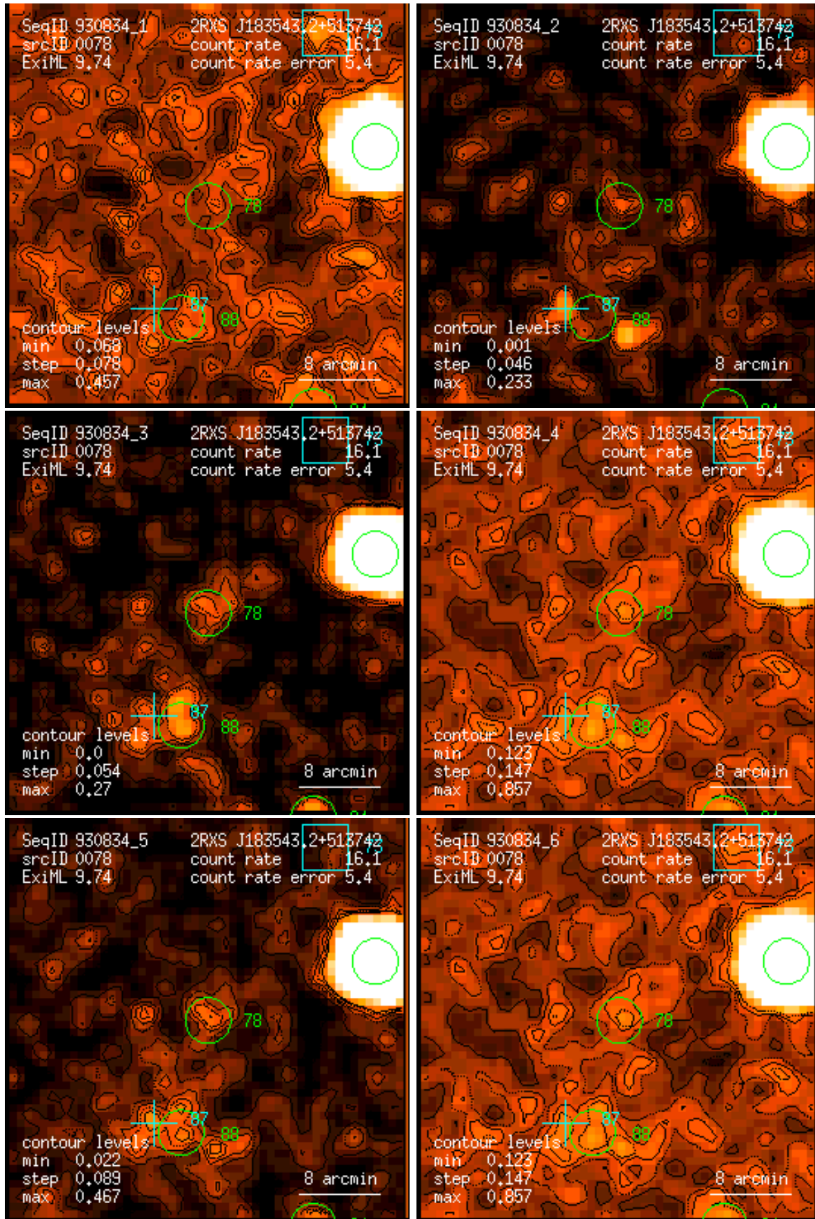
Figure 78: RASS 930834: detection 0078: band rate images, Gaussian filter: (1) PSPC channels 11 – 41, (2) 52 – 90, (3) 91 – 201, (4) 11 – 235, (5) 52 – 201, (6) 11 – 201. Broad band rates in counts/ks. Band rate contour levels in counts/ks/arcmin 2 .
