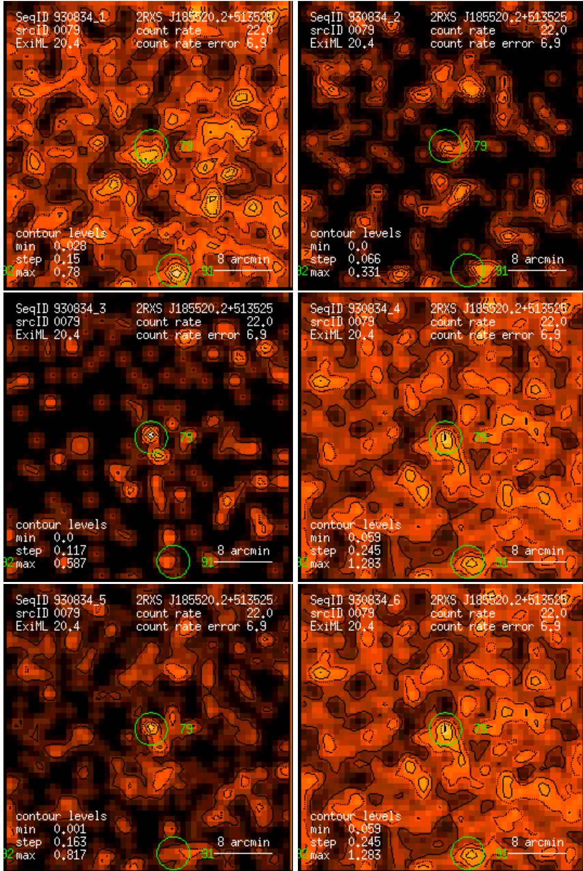
Figure 79: RASS 930834: detection 0079: band rate images, Gaussian filter: (1) PSPC channels 11 – 41, (2) 52 – 90, (3) 91 – 201, (4) 11 – 235, (5) 52 – 201, (6) 11 – 201. Broad band rates in counts/ks. Band rate contour levels in counts/ks/arcmin 2 .
