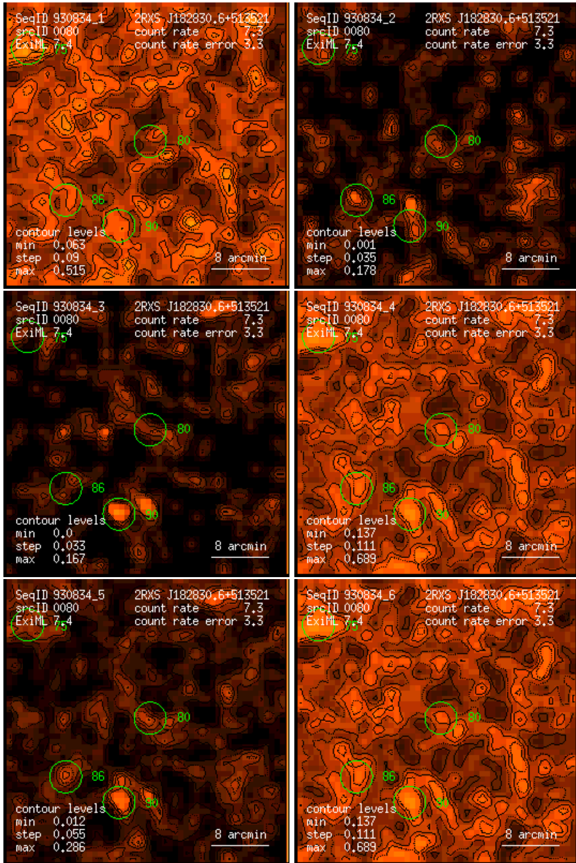
Figure 80: RASS 930834: detection 0080: band rate images, Gaussian filter: (1) PSPC channels 11 – 41, (2) 52 – 90, (3) 91 – 201, (4) 11 – 235, (5) 52 – 201, (6) 11 – 201. Broad band rates in counts/ks. Band rate contour levels in counts/ks/arcmin 2 .
