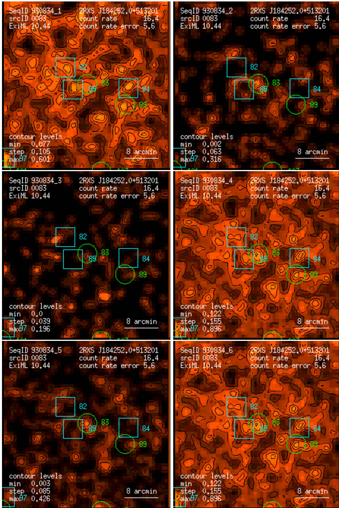
Figure 83: RASS 930834: detection 0083: band rate images, Gaussian filter: (1) PSPC channels 11 – 41, (2) 52 – 90, (3) 91 – 201, (4) 11 – 235, (5) 52 – 201, (6) 11 – 201. Broad band rates in counts/ks. Band rate contour levels in counts/ks/arcmin 2 .
