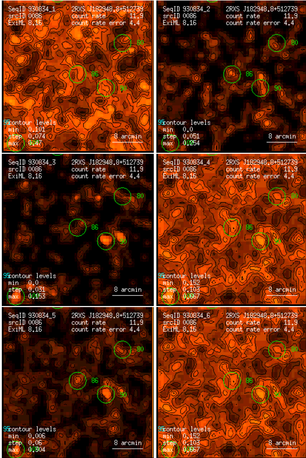
Figure 86: RASS 930834: detection 0086: band rate images, Gaussian filter: (1) PSPC channels 11 – 41, (2) 52 – 90, (3) 91 – 201, (4) 11 – 235, (5) 52 – 201, (6) 11 – 201. Broad band rates in counts/ks. Band rate contour levels in counts/ks/arcmin 2 .
