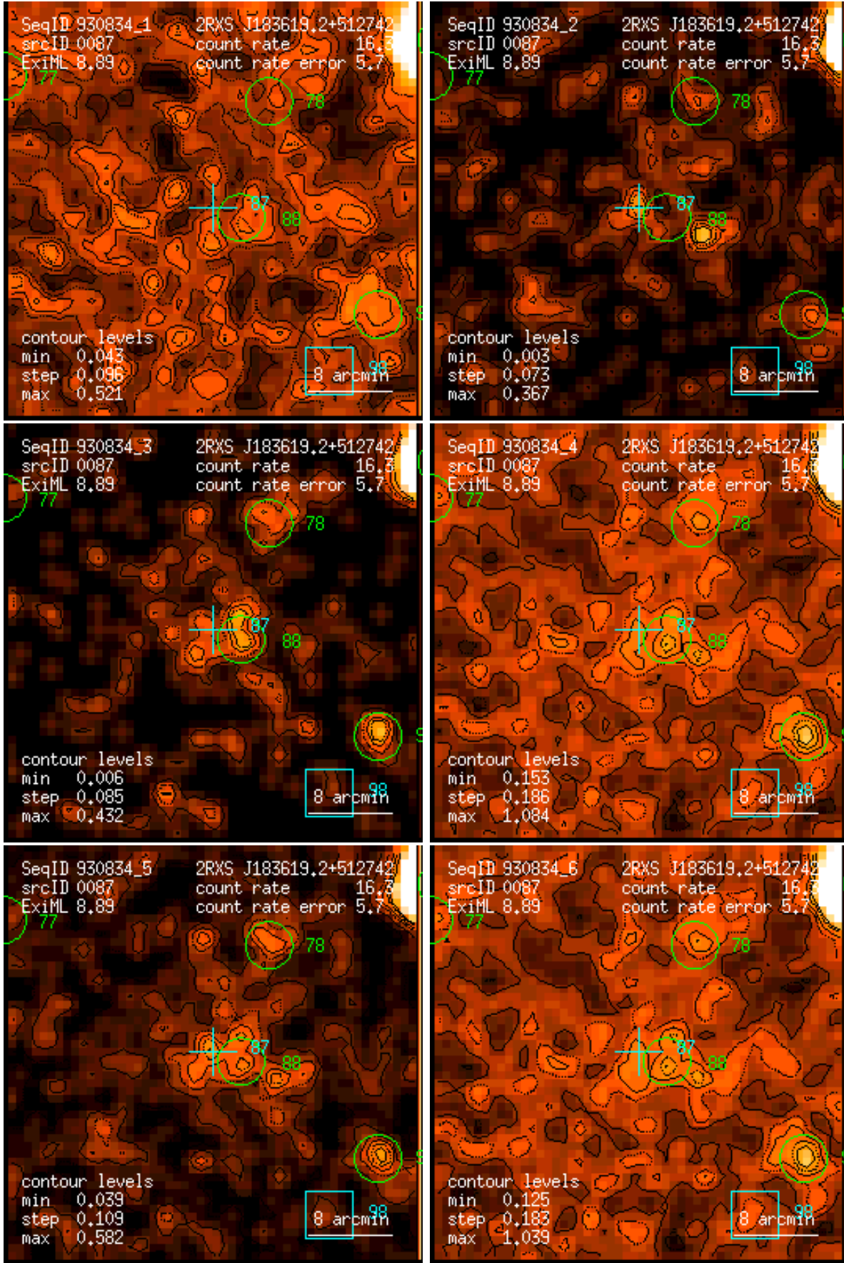
Figure 87: RASS 930834: detection 0087: band rate images, Gaussian filter: (1) PSPC channels 11 – 41, (2) 52 – 90, (3) 91 – 201, (4) 11 – 235, (5) 52 – 201, (6) 11 – 201. Broad band rates in counts/ks. Band rate contour levels in counts/ks/arcmin 2 .
