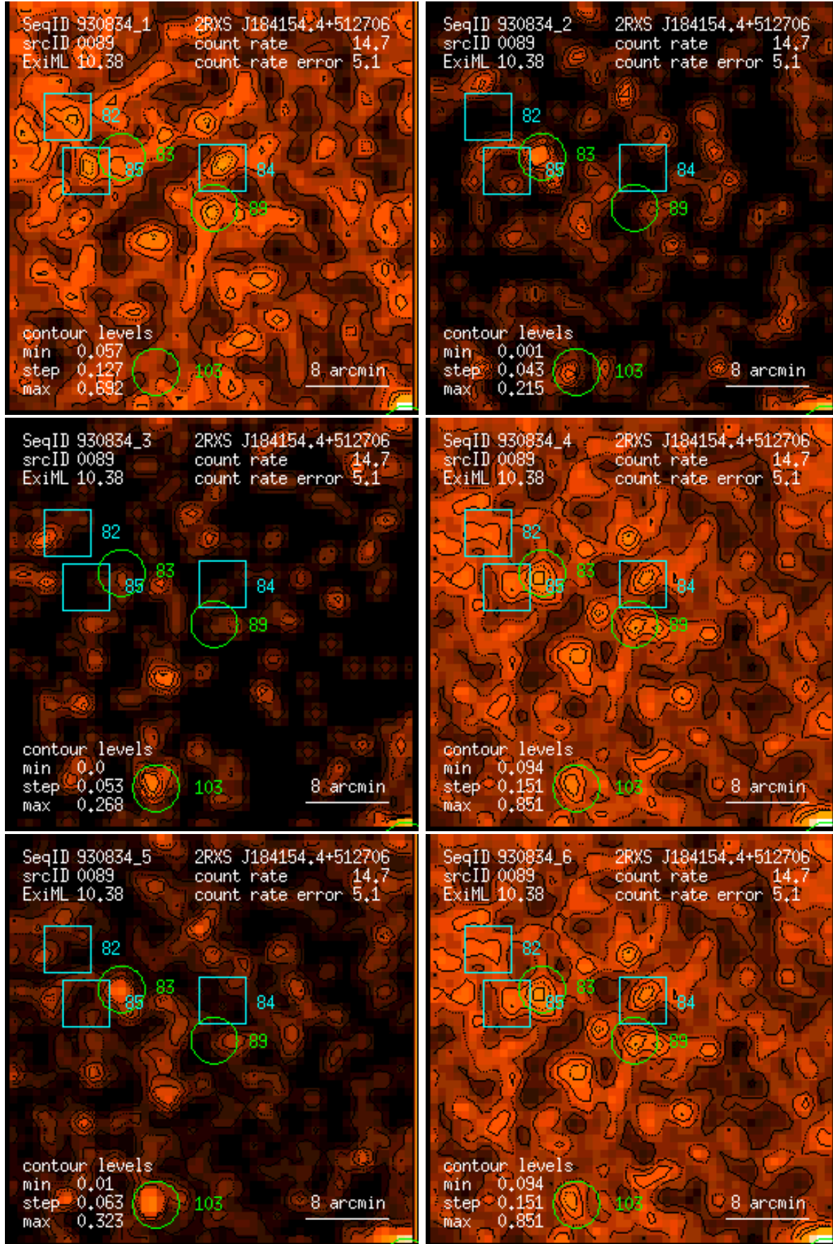
Figure 89: RASS 930834: detection 0089: band rate images, Gaussian filter: (1) PSPC channels 11 – 41, (2) 52 – 90, (3) 91 – 201, (4) 11 – 235, (5) 52 – 201, (6) 11 – 201. Broad band rates in counts/ks. Band rate contour levels in counts/ks/arcmin 2 .
