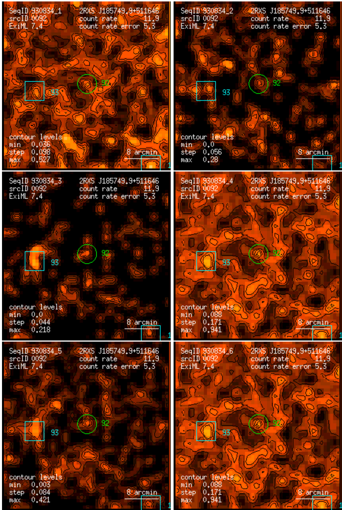
Figure 92: RASS 930834: detection 0092: band rate images, Gaussian filter: (1) PSPC channels 11 – 41, (2) 52 – 90, (3) 91 – 201, (4) 11 – 235, (5) 52 – 201, (6) 11 – 201. Broad band rates in counts/ks. Band rate contour levels in counts/ks/arcmin 2 .
