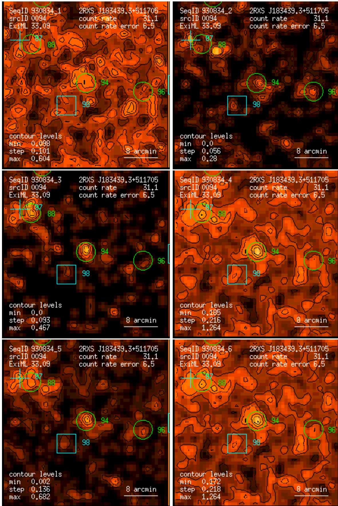
Figure 94: RASS 930834: detection 0094: band rate images, Gaussian filter: (1) PSPC channels 11 – 41, (2) 52 – 90, (3) 91 – 201, (4) 11 – 235, (5) 52 – 201, (6) 11 – 201. Broad band rates in counts/ks. Band rate contour levels in counts/ks/arcmin 2 .
