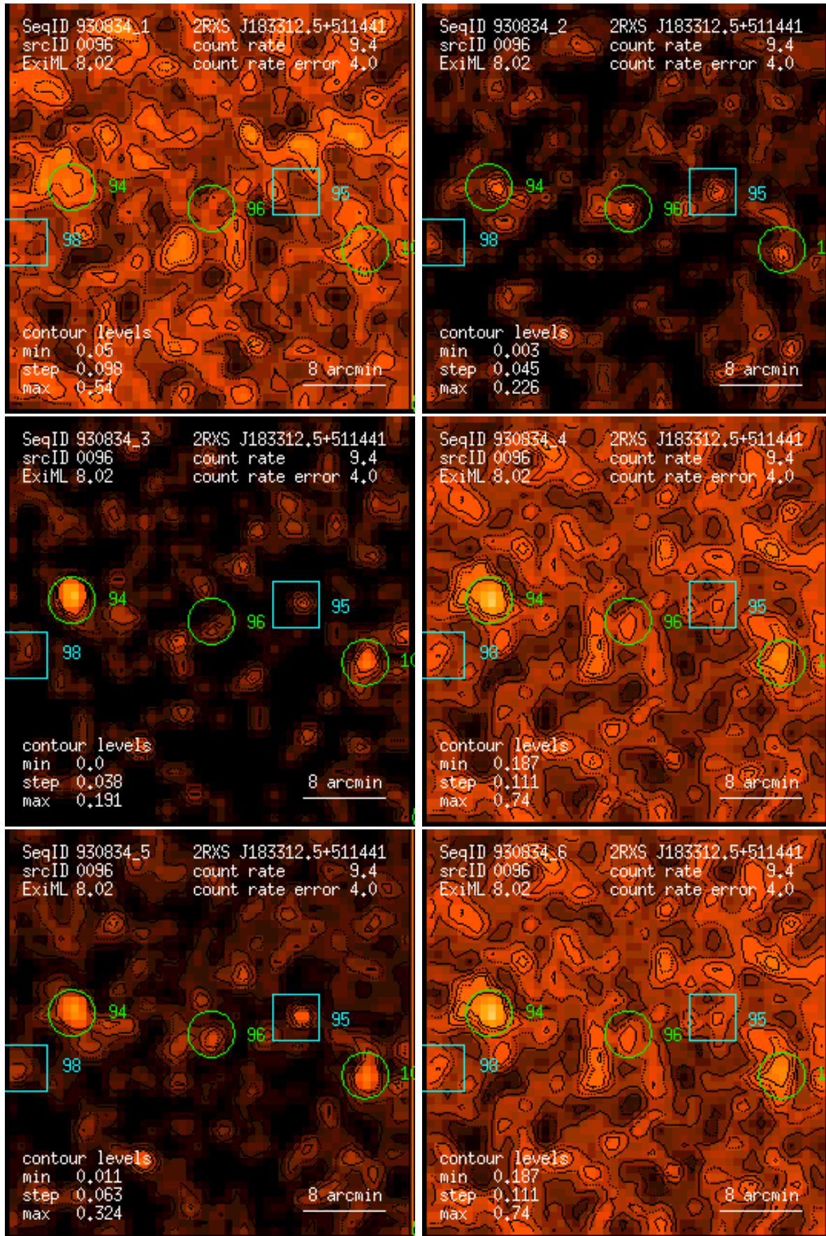
Figure 96: RASS 930834: detection 0096: band rate images, Gaussian filter: (1) PSPC channels 11 – 41, (2) 52 – 90, (3) 91 – 201, (4) 11 – 235, (5) 52 – 201, (6) 11 – 201. Broad band rates in counts/ks. Band rate contour levels in counts/ks/arcmin 2 .
