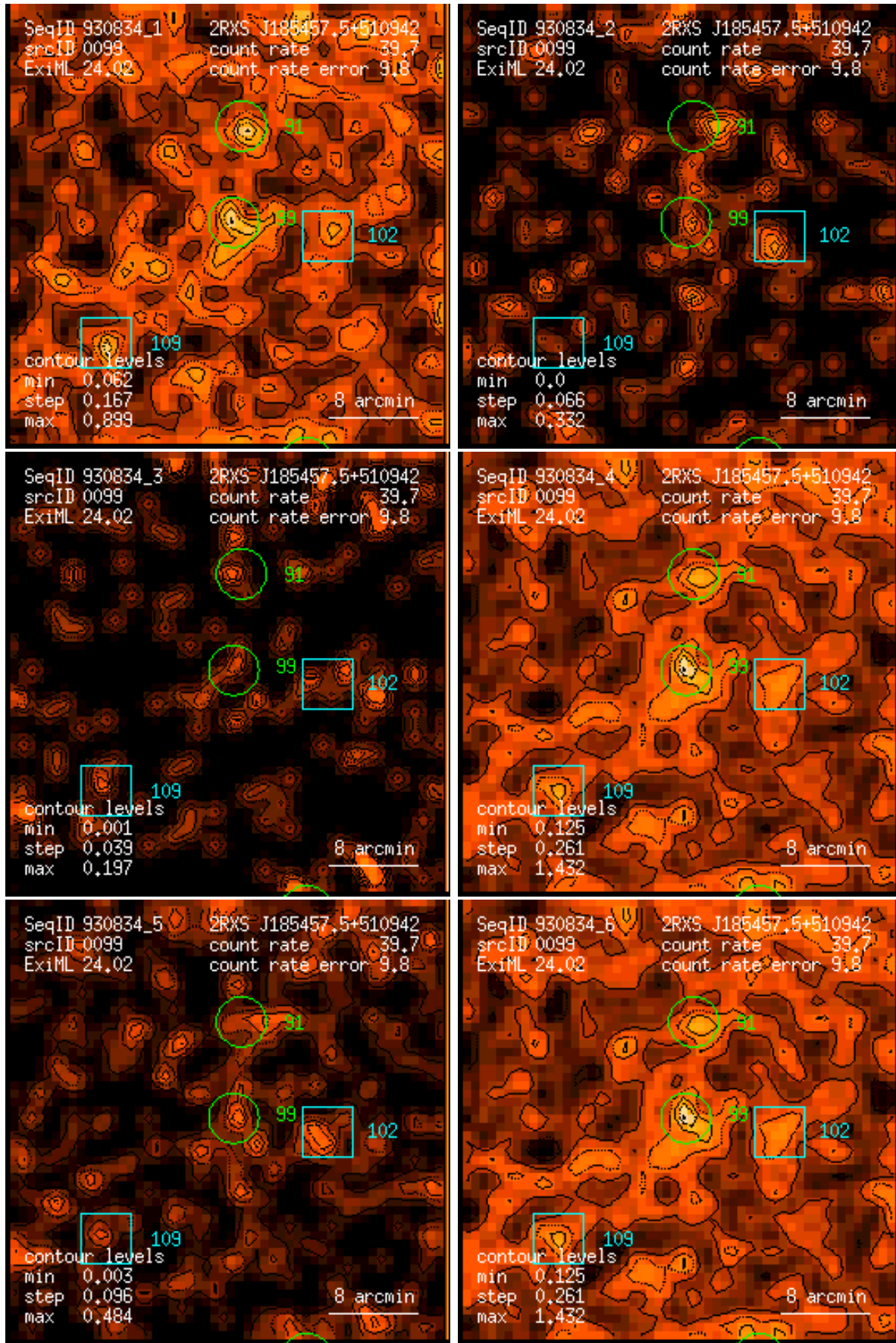
Figure 99: RASS 930834: detection 0099: band rate images, Gaussian filter: (1) PSPC channels 11 – 41, (2) 52 – 90, (3) 91 – 201, (4) 11 – 235, (5) 52 – 201, (6) 11 – 201. Broad band rates in counts/ks. Band rate contour levels in counts/ks/arcmin 2 .
