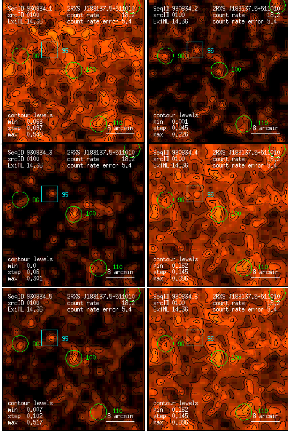
Figure 100: RASS 930834: detection 0100: band rate images, Gaussian filter: (1) PSPC channels 11 – 41, (2) 52 – 90, (3) 91 – 201, (4) 11 – 235, (5) 52 – 201, (6) 11 – 201. Broad band rates in counts/ks. Band rate contour levels in counts/ks/arcmin 2 .
