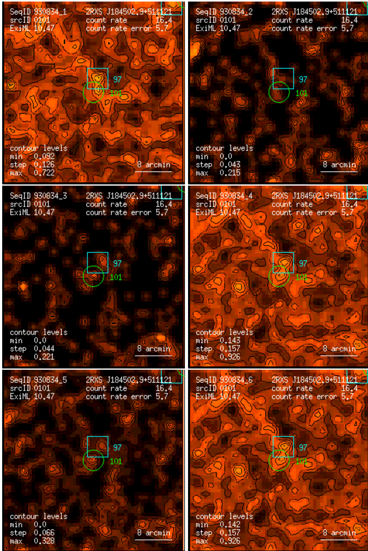
Figure 101: RASS 930834: detection 0101: band rate images, Gaussian filter: (1) PSPC channels 11 – 41, (2) 52 – 90, (3) 91 – 201, (4) 11 – 235, (5) 52 – 201, (6) 11 – 201. Broad band rates in counts/ks. Band rate contour levels in counts/ks/arcmin 2 .
