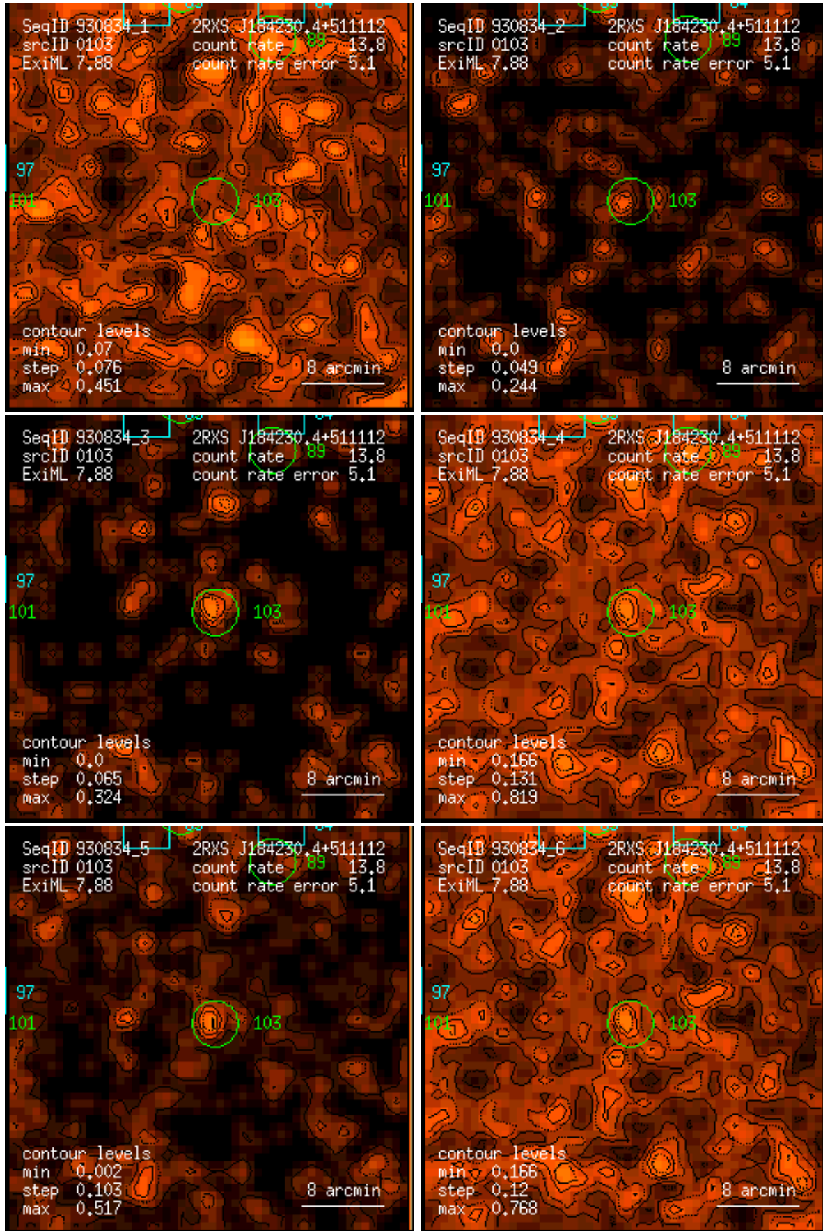
Figure 103: RASS 930834: detection 0103: band rate images, Gaussian filter: (1) PSPC channels 11 – 41, (2) 52 – 90, (3) 91 – 201, (4) 11 – 235, (5) 52 – 201, (6) 11 – 201. Broad band rates in counts/ks. Band rate contour levels in counts/ks/arcmin 2 .
