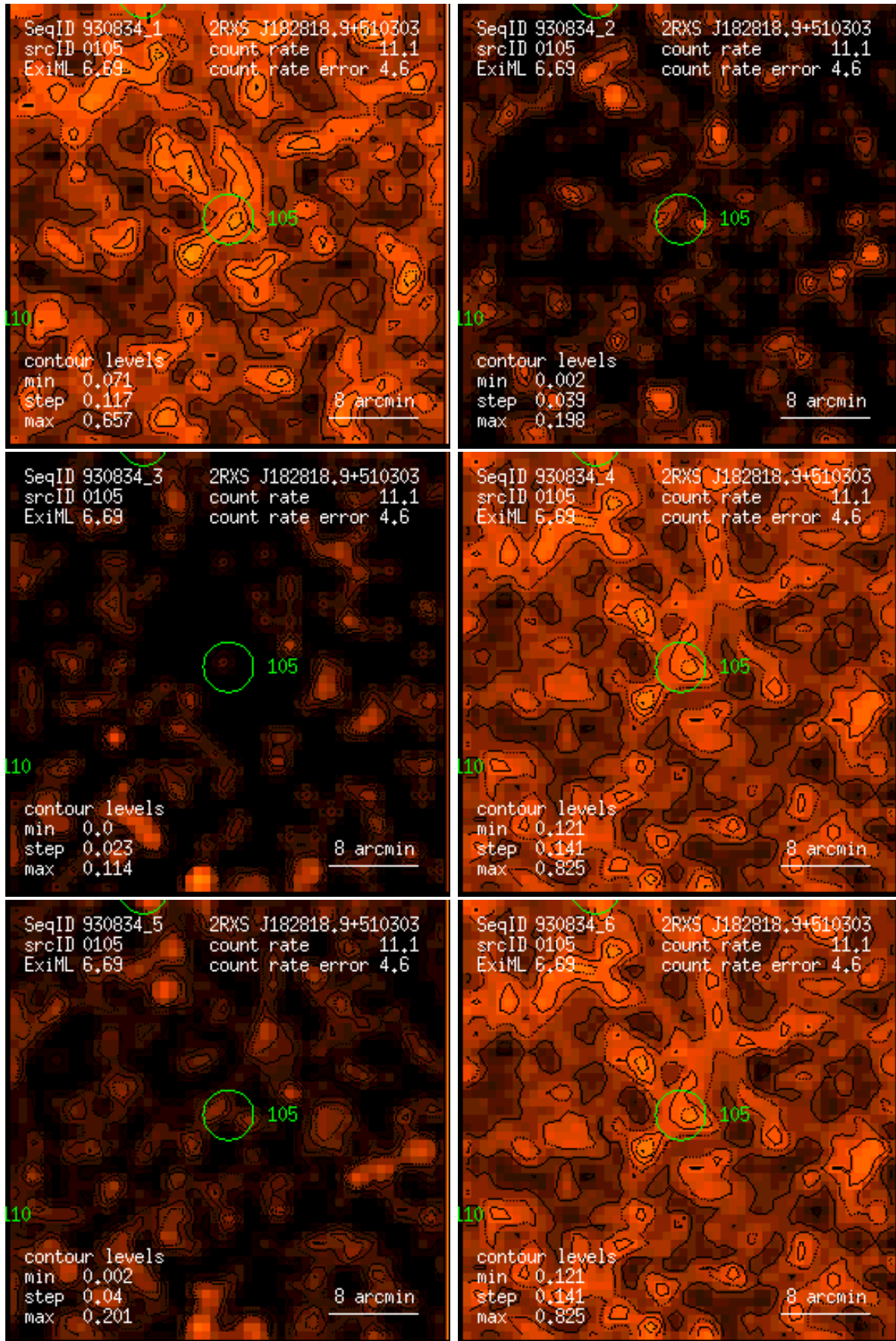
Figure 105: RASS 930834: detection 0105: band rate images, Gaussian filter: (1) PSPC channels 11 – 41, (2) 52 – 90, (3) 91 – 201, (4) 11 – 235, (5) 52 – 201, (6) 11 – 201. Broad band rates in counts/ks. Band rate contour levels in counts/ks/arcmin 2 .
