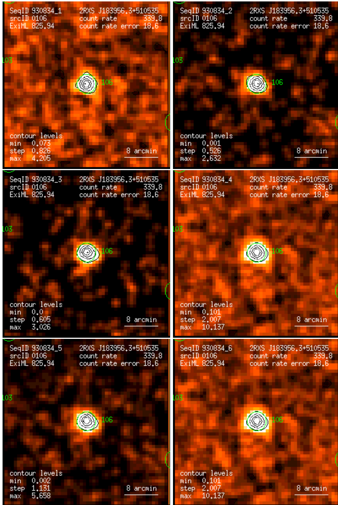
Figure 106: RASS 930834: detection 0106: band rate images, Gaussian filter: (1) PSPC channels 11 – 41, (2) 52 – 90, (3) 91 – 201, (4) 11 – 235, (5) 52 – 201, (6) 11 – 201. Broad band rates in counts/ks. Band rate contour levels in counts/ks/arcmin 2 .
