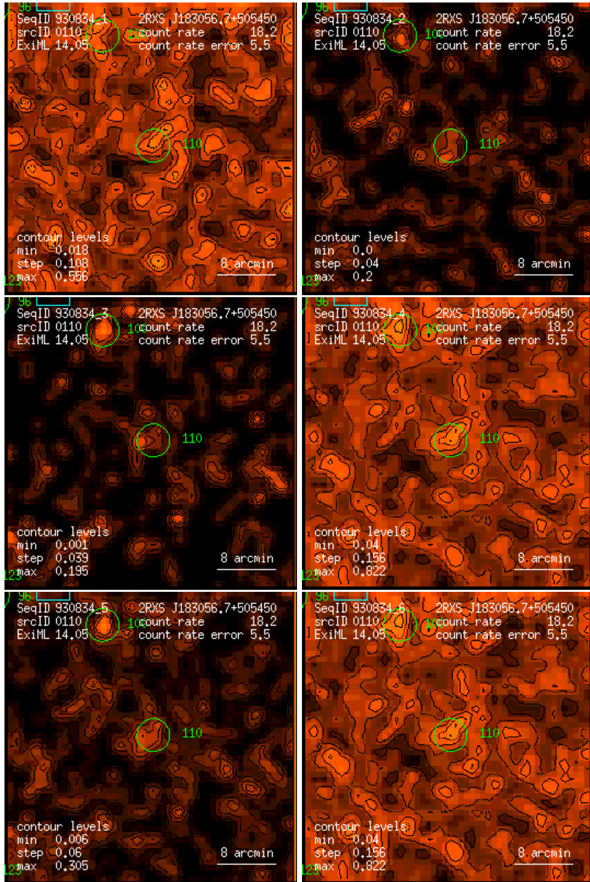
Figure 110: RASS 930834: detection 0110: band rate images, Gaussian filter: (1) PSPC channels 11 – 41, (2) 52 – 90, (3) 91 – 201, (4) 11 – 235, (5) 52 – 201, (6) 11 – 201. Broad band rates in counts/ks. Band rate contour levels in counts/ks/arcmin 2 .
