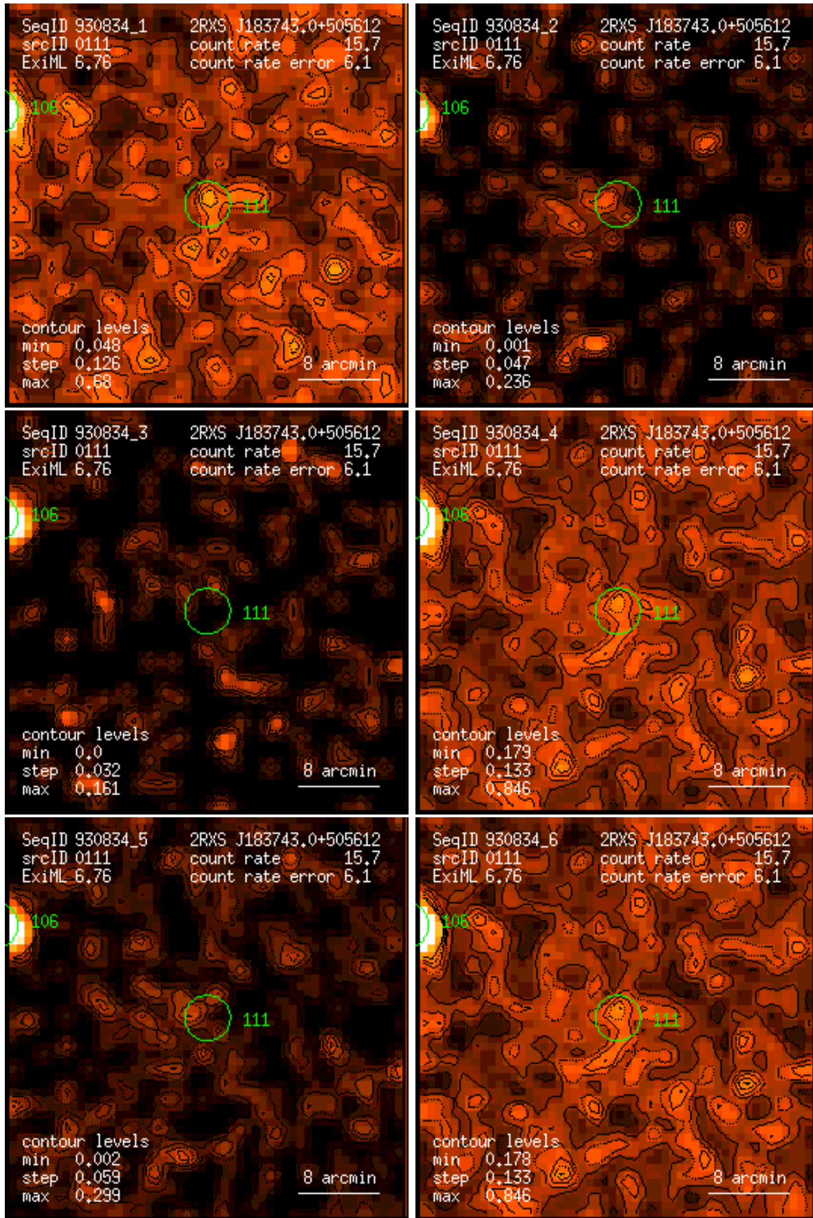
Figure 111: RASS 930834: detection 0111: band rate images, Gaussian filter: (1) PSPC channels 11 – 41, (2) 52 – 90, (3) 91 – 201, (4) 11 – 235, (5) 52 – 201, (6) 11 – 201. Broad band rates in counts/ks. Band rate contour levels in counts/ks/arcmin 2 .
