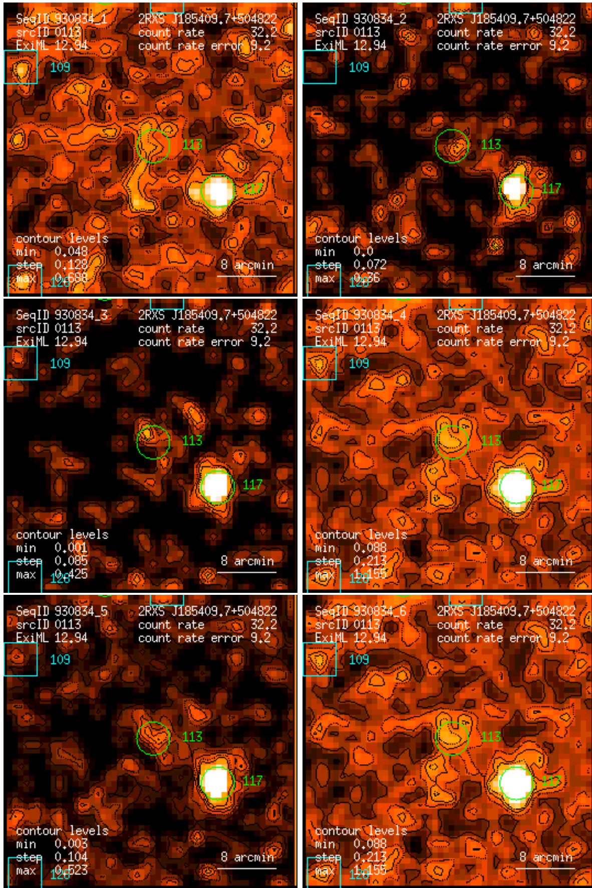
Figure 113: RASS 930834: detection 0113: band rate images, Gaussian filter: (1) PSPC channels 11 – 41, (2) 52 – 90, (3) 91 – 201, (4) 11 – 235, (5) 52 – 201, (6) 11 – 201. Broad band rates in counts/ks. Band rate contour levels in counts/ks/arcmin 2 .
