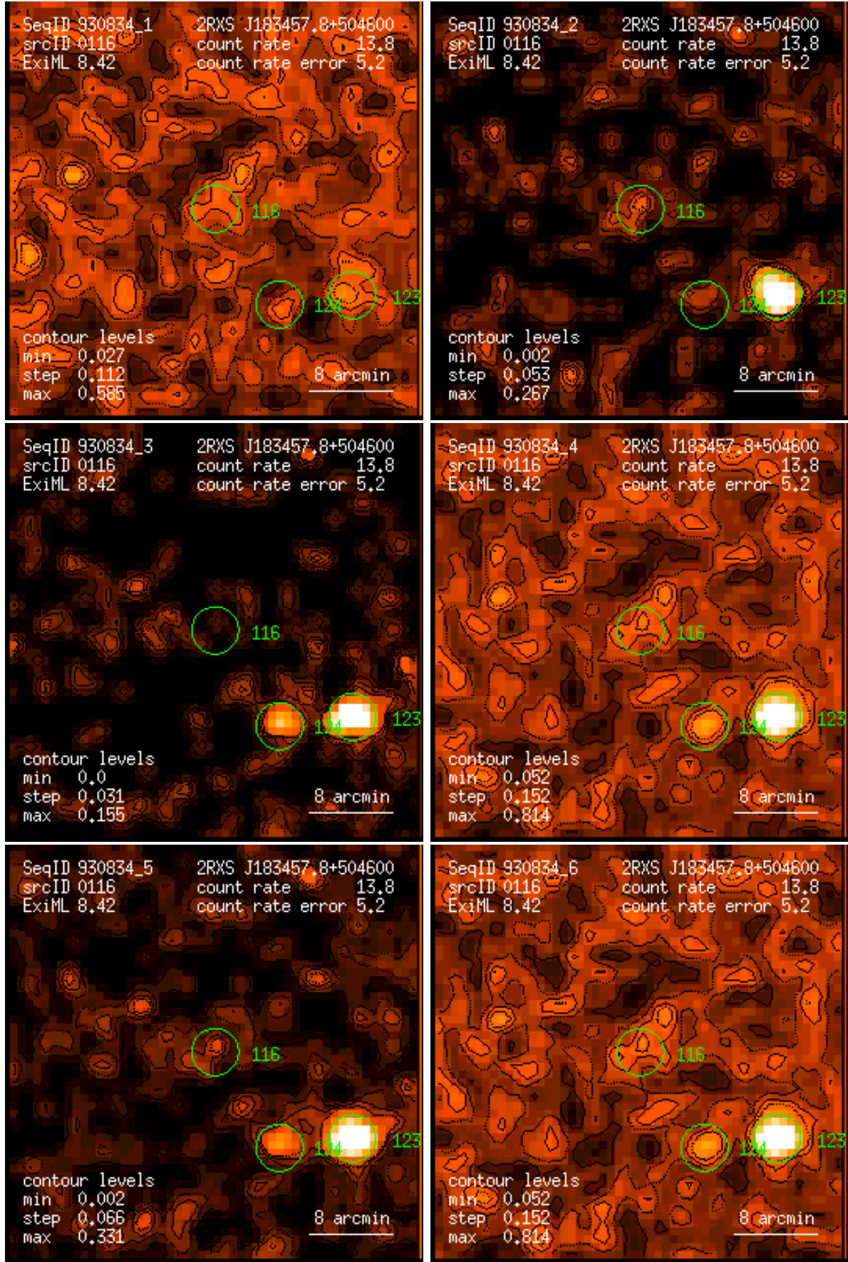
Figure 116: RASS 930834: detection 0116: band rate images, Gaussian filter: (1) PSPC channels 11 – 41, (2) 52 – 90, (3) 91 – 201, (4) 11 – 235, (5) 52 – 201, (6) 11 – 201. Broad band rates in counts/ks. Band rate contour levels in counts/ks/arcmin 2 .
