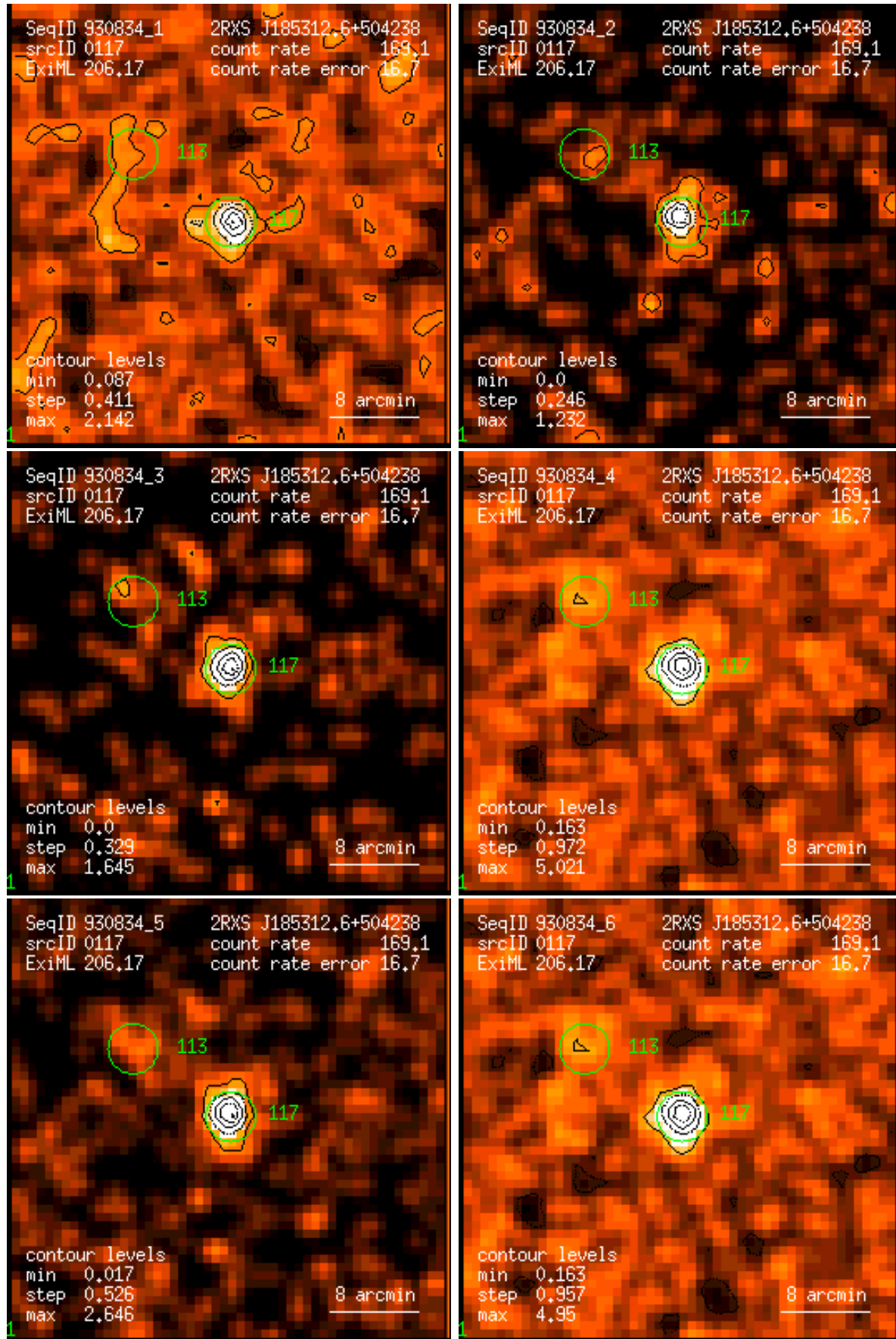
Figure 117: RASS 930834: detection 0117: band rate images, Gaussian filter: (1) PSPC channels 11 – 41, (2) 52 – 90, (3) 91 – 201, (4) 11 – 235, (5) 52 – 201, (6) 11 – 201. Broad band rates in counts/ks. Band rate contour levels in counts/ks/arcmin 2 .
