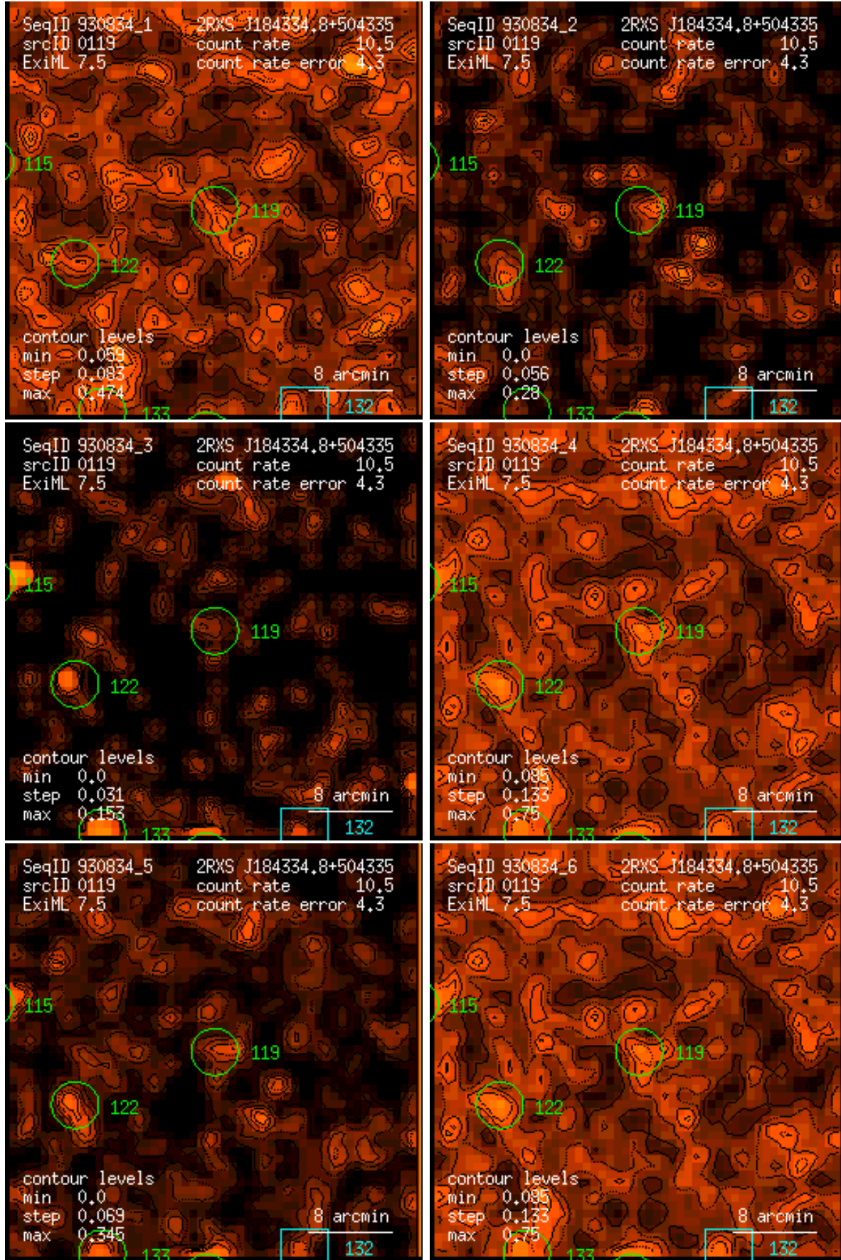
Figure 119: RASS 930834: detection 0119: band rate images, Gaussian filter: (1) PSPC channels 11 – 41, (2) 52 – 90, (3) 91 – 201, (4) 11 – 235, (5) 52 – 201, (6) 11 – 201. Broad band rates in counts/ks. Band rate contour levels in counts/ks/arcmin 2 .
