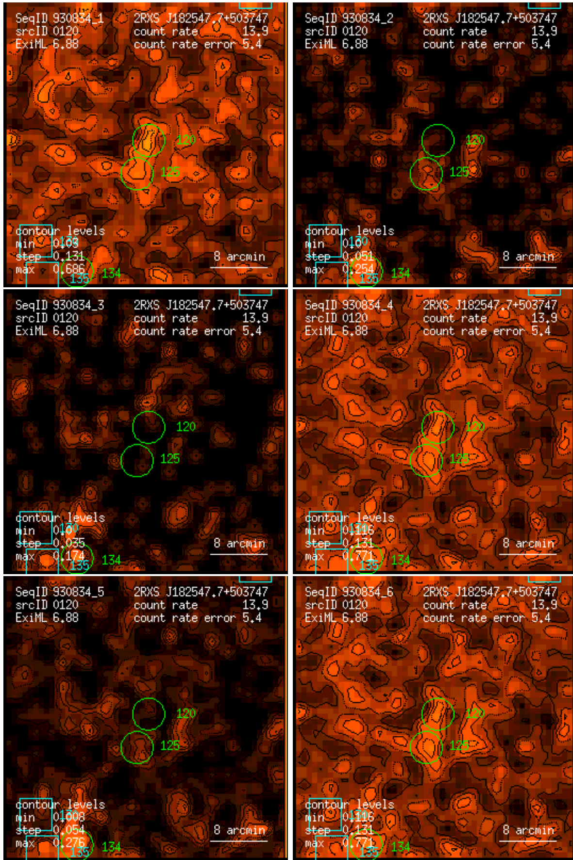
Figure 120: RASS 930834: detection 0120: band rate images, Gaussian filter: (1) PSPC channels 11 – 41, (2) 52 – 90, (3) 91 – 201, (4) 11 – 235, (5) 52 – 201, (6) 11 – 201. Broad band rates in counts/ks. Band rate contour levels in counts/ks/arcmin 2 .
