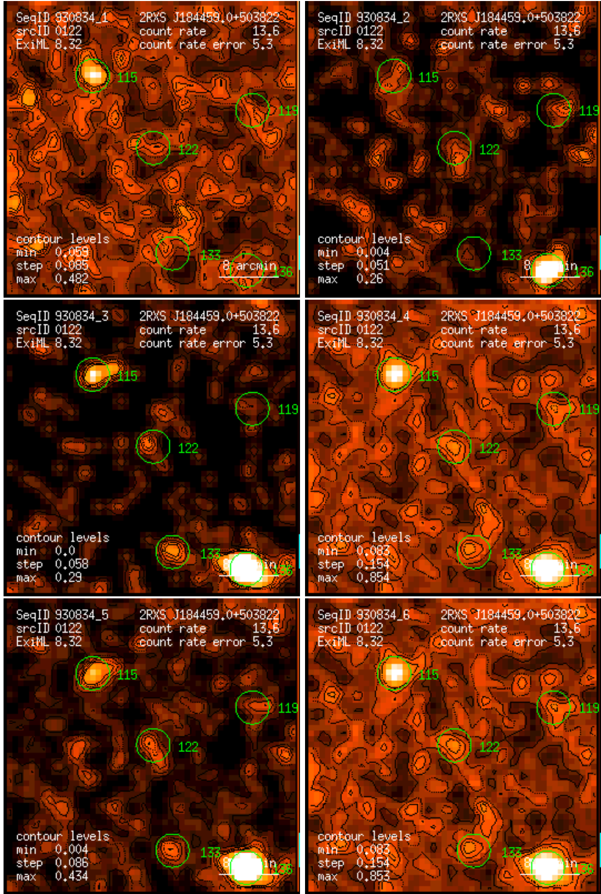
Figure 122: RASS 930834: detection 0122: band rate images, Gaussian filter: (1) PSPC channels 11 – 41, (2) 52 – 90, (3) 91 – 201, (4) 11 – 235, (5) 52 – 201, (6) 11 – 201. Broad band rates in counts/ks. Band rate contour levels in counts/ks/arcmin 2 .
