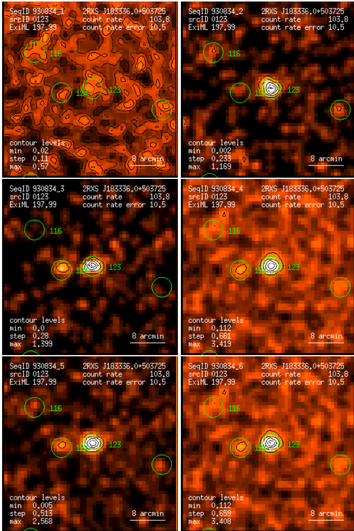
Figure 123: RASS 930834: detection 0123: band rate images, Gaussian filter: (1) PSPC channels 11 – 41, (2) 52 – 90, (3) 91 – 201, (4) 11 – 235, (5) 52 – 201, (6) 11 – 201. Broad band rates in counts/ks. Band rate contour levels in counts/ks/arcmin 2 .
