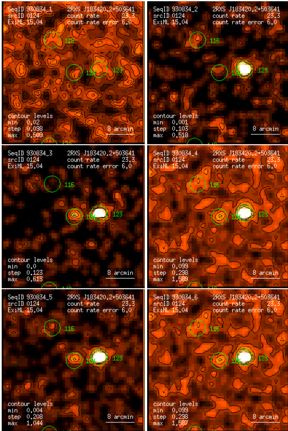
Figure 124: RASS 930834: detection 0124: band rate images, Gaussian filter: (1) PSPC channels 11 – 41, (2) 52 – 90, (3) 91 – 201, (4) 11 – 235, (5) 52 – 201, (6) 11 – 201. Broad band rates in counts/ks. Band rate contour levels in counts/ks/arcmin 2 .
