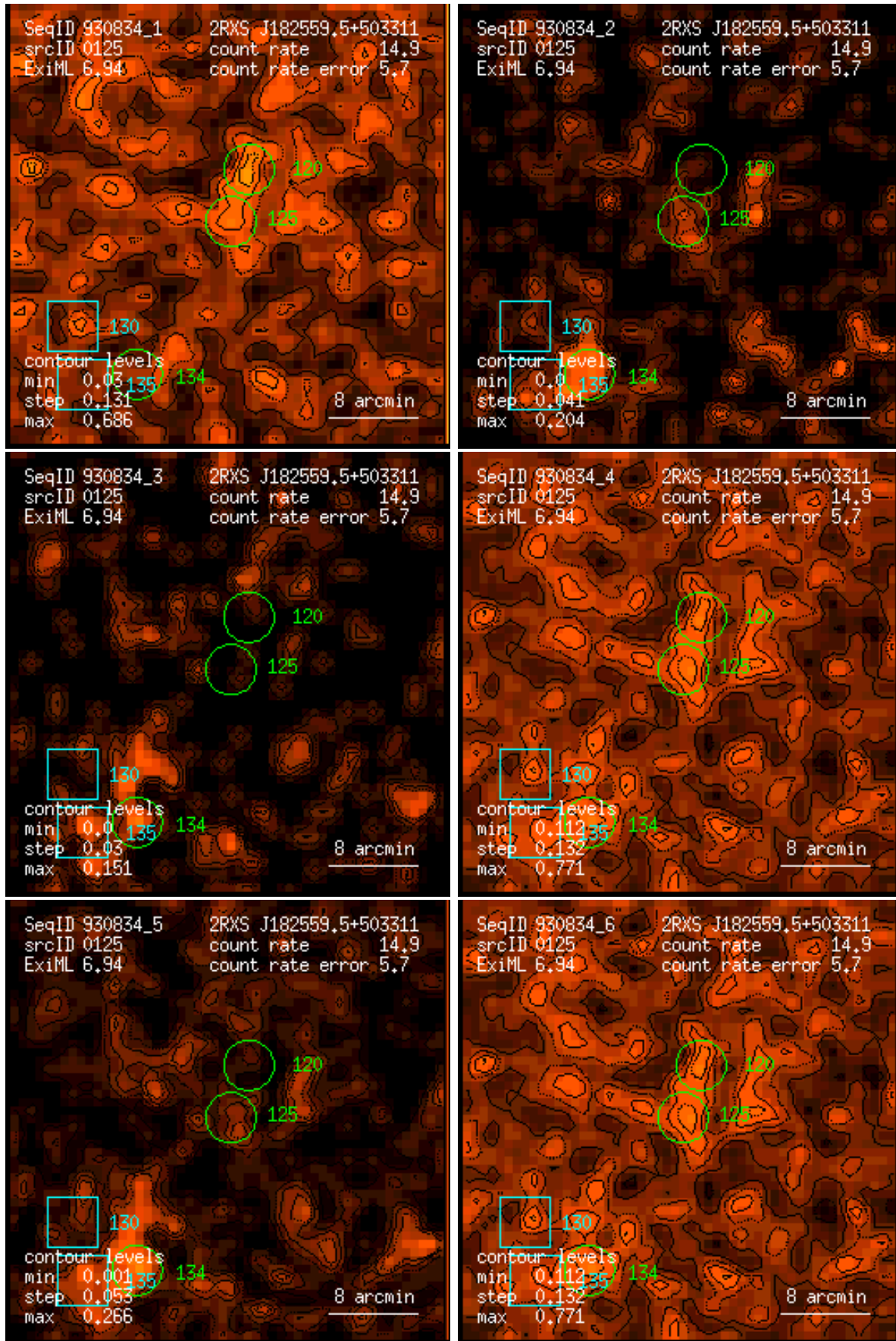
Figure 125: RASS 930834: detection 0125: band rate images, Gaussian filter: (1) PSPC channels 11 – 41, (2) 52 – 90, (3) 91 – 201, (4) 11 – 235, (5) 52 – 201, (6) 11 – 201. Broad band rates in counts/ks. Band rate contour levels in counts/ks/arcmin 2 .
