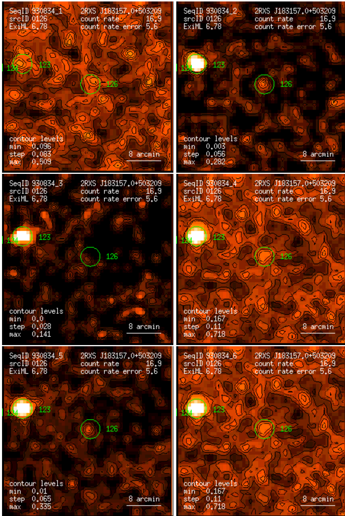
Figure 126: RASS 930834: detection 0126: band rate images, Gaussian filter: (1) PSPC channels 11 – 41, (2) 52 – 90, (3) 91 – 201, (4) 11 – 235, (5) 52 – 201, (6) 11 – 201. Broad band rates in counts/ks. Band rate contour levels in counts/ks/arcmin 2 .
