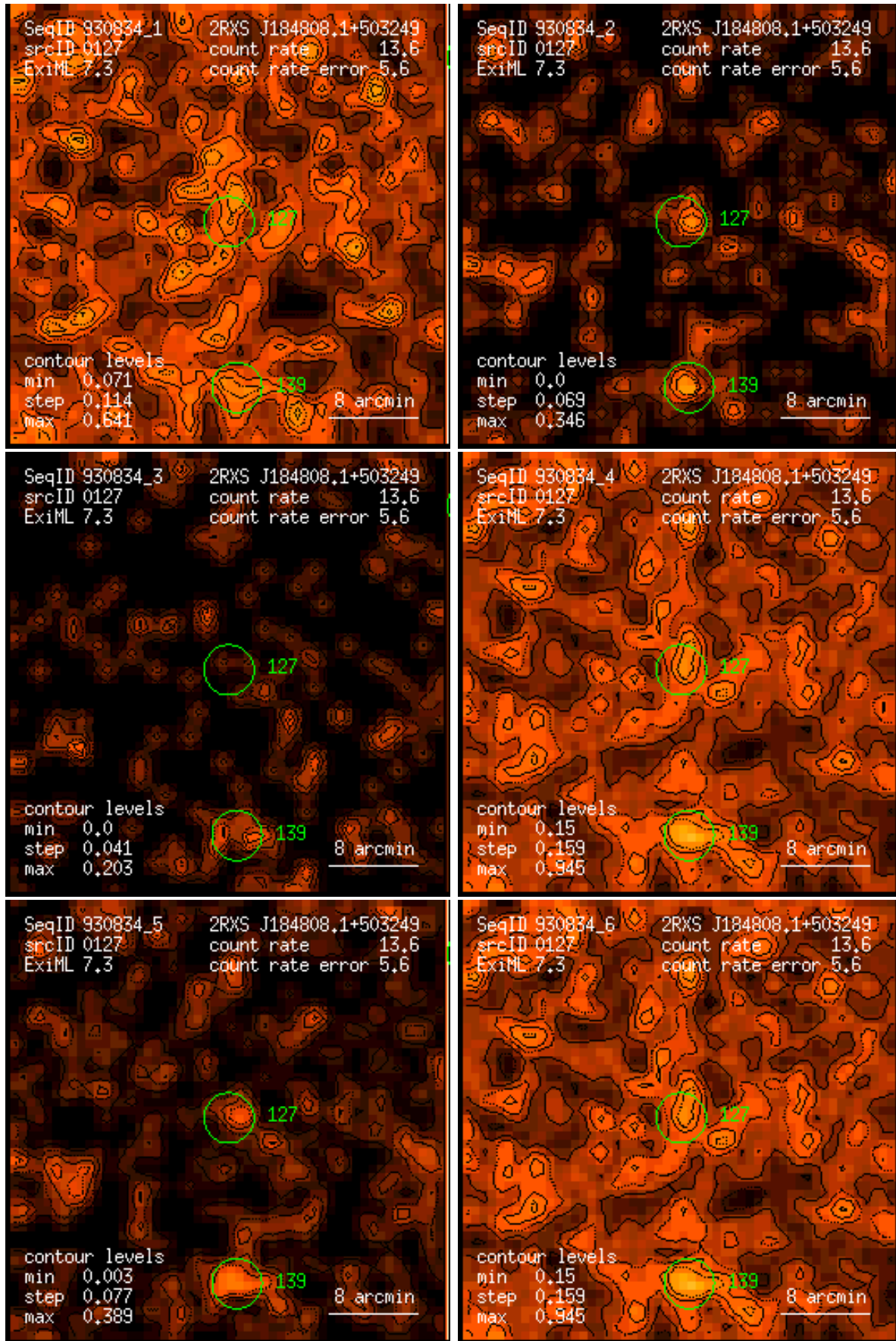
Figure 127: RASS 930834: detection 0127: band rate images, Gaussian filter: (1) PSPC channels 11 – 41, (2) 52 – 90, (3) 91 – 201, (4) 11 – 235, (5) 52 – 201, (6) 11 – 201. Broad band rates in counts/ks. Band rate contour levels in counts/ks/arcmin 2 .
