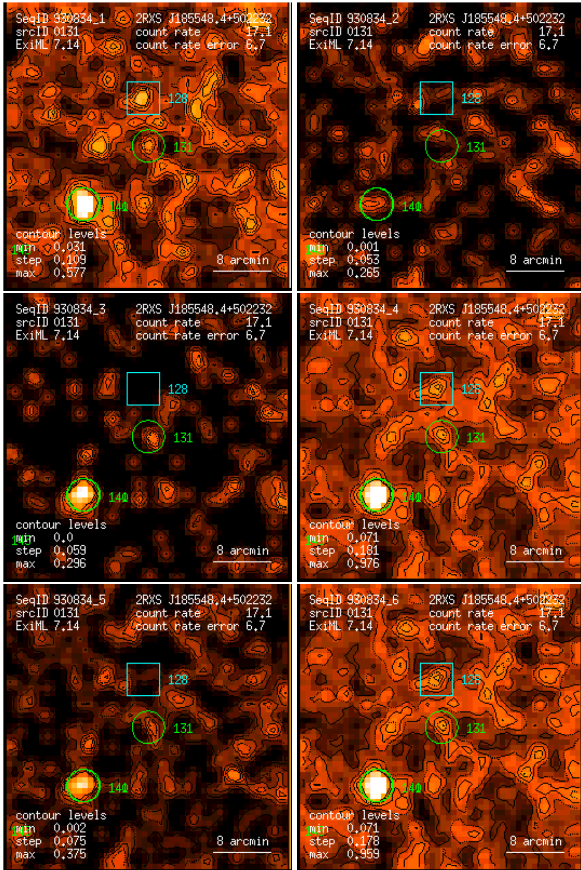
Figure 131: RASS 930834: detection 0131: band rate images, Gaussian filter: (1) PSPC channels 11 – 41, (2) 52 – 90, (3) 91 – 201, (4) 11 – 235, (5) 52 – 201, (6) 11 – 201. Broad band rates in counts/ks. Band rate contour levels in counts/ks/arcmin 2 .
