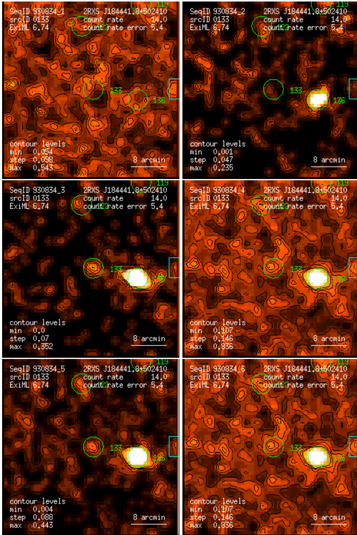
Figure 133: RASS 930834: detection 0133: band rate images, Gaussian filter: (1) PSPC channels 11 – 41, (2) 52 – 90, (3) 91 – 201, (4) 11 – 235, (5) 52 – 201, (6) 11 – 201. Broad band rates in counts/ks. Band rate contour levels in counts/ks/arcmin 2 .
