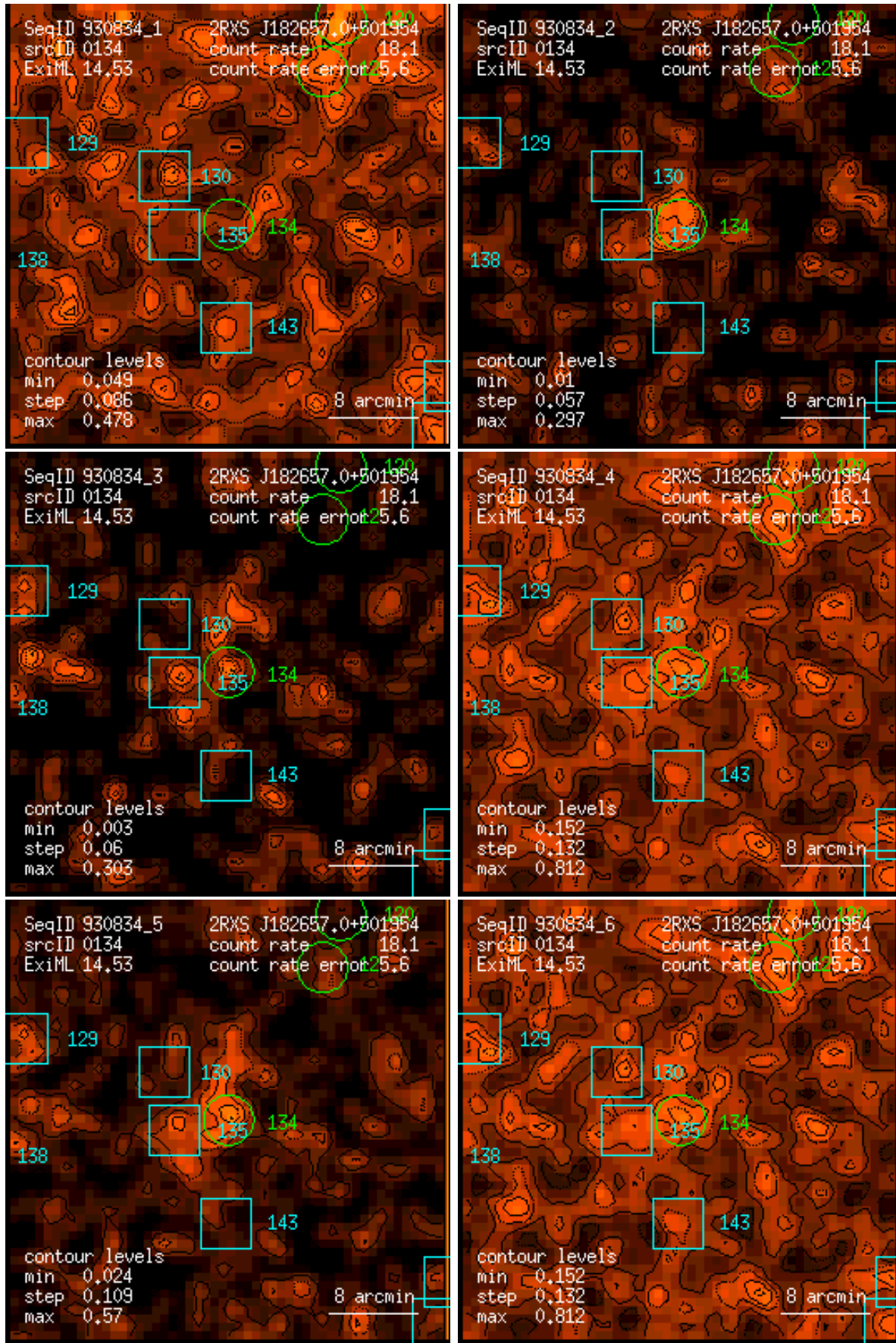
Figure 134: RASS 930834: detection 0134: band rate images, Gaussian filter: (1) PSPC channels 11 – 41, (2) 52 – 90, (3) 91 – 201, (4) 11 – 235, (5) 52 – 201, (6) 11 – 201. Broad band rates in counts/ks. Band rate contour levels in counts/ks/arcmin 2 .
