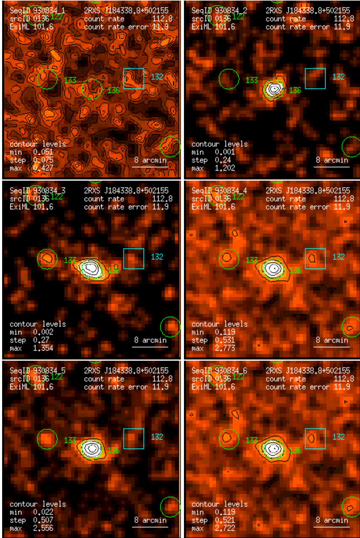
Figure 136: RASS 930834: detection 0136: band rate images, Gaussian filter: (1) PSPC channels 11 – 41, (2) 52 – 90, (3) 91 – 201, (4) 11 – 235, (5) 52 – 201, (6) 11 – 201. Broad band rates in counts/ks. Band rate contour levels in counts/ks/arcmin 2 .
