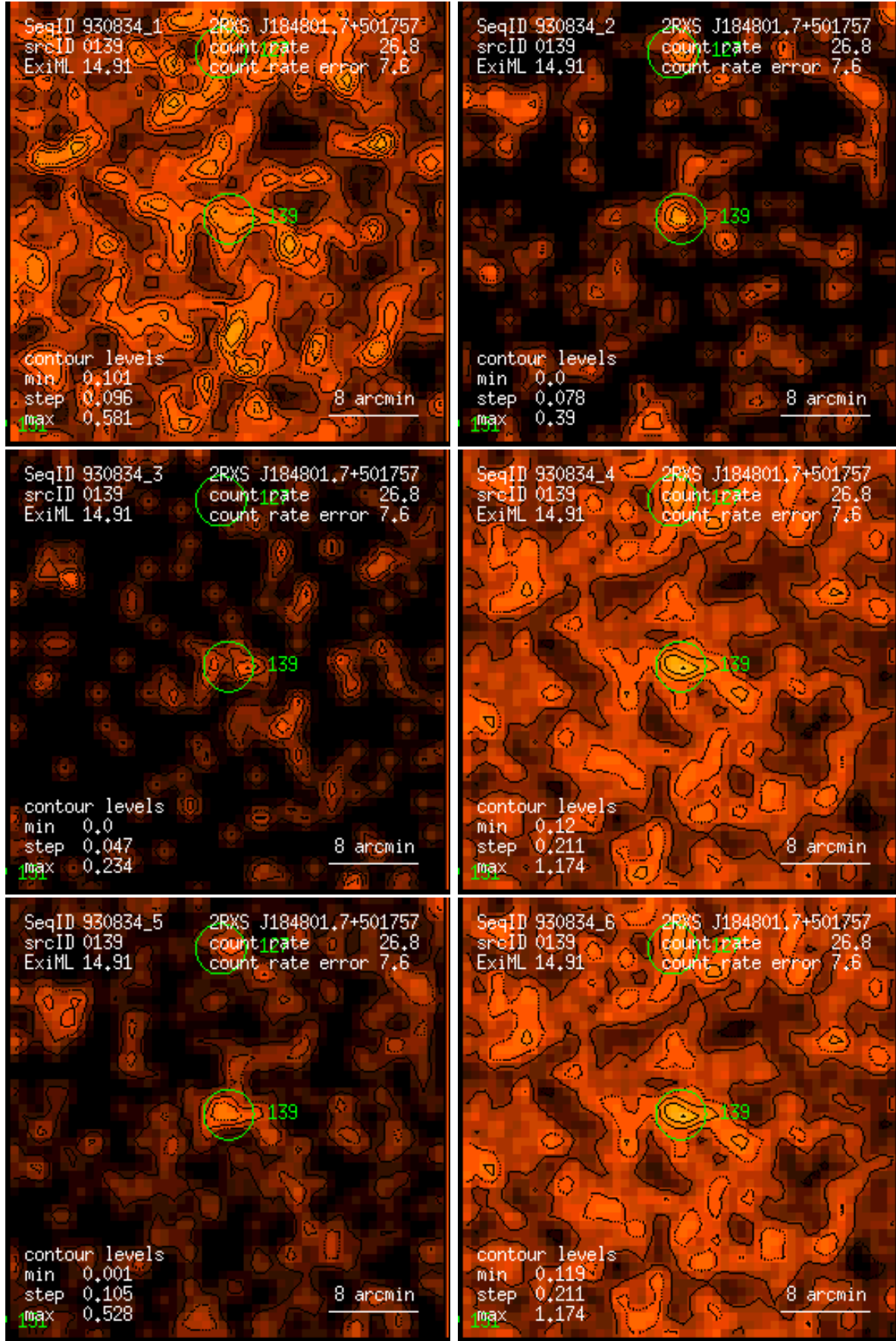
Figure 139: RASS 930834: detection 0139: band rate images, Gaussian filter: (1) PSPC channels 11 – 41, (2) 52 – 90, (3) 91 – 201, (4) 11 – 235, (5) 52 – 201, (6) 11 – 201. Broad band rates in counts/ks. Band rate contour levels in counts/ks/arcmin 2 .
