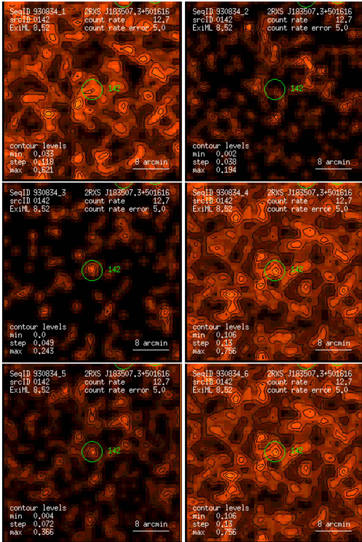
Figure 142: RASS 930834: detection 0142: band rate images, Gaussian filter: (1) PSPC channels 11 – 41, (2) 52 – 90, (3) 91 – 201, (4) 11 – 235, (5) 52 – 201, (6) 11 – 201. Broad band rates in counts/ks. Band rate contour levels in counts/ks/arcmin 2 .
