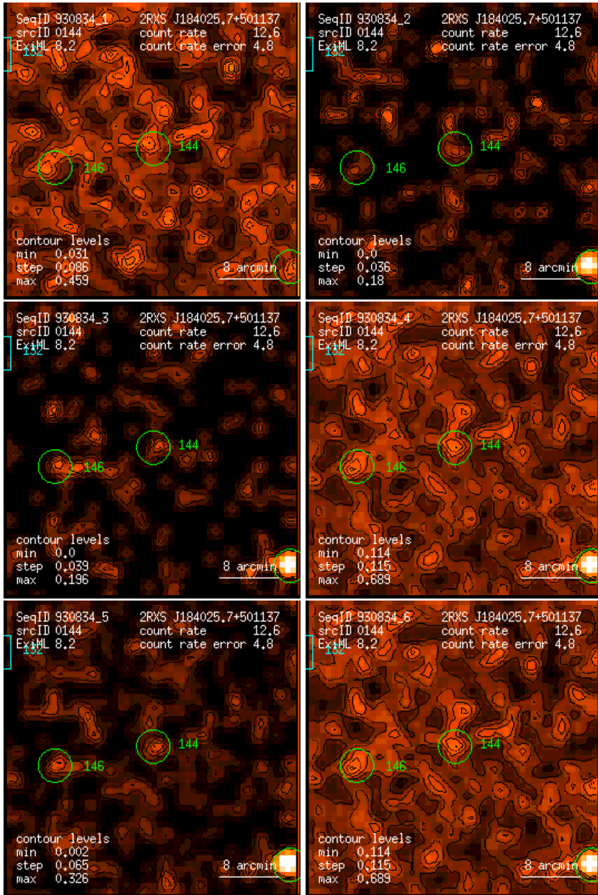
Figure 144: RASS 930834: detection 0144: band rate images, Gaussian filter: (1) PSPC channels 11 – 41, (2) 52 – 90, (3) 91 – 201, (4) 11 – 235, (5) 52 – 201, (6) 11 – 201. Broad band rates in counts/ks. Band rate contour levels in counts/ks/arcmin 2 .
