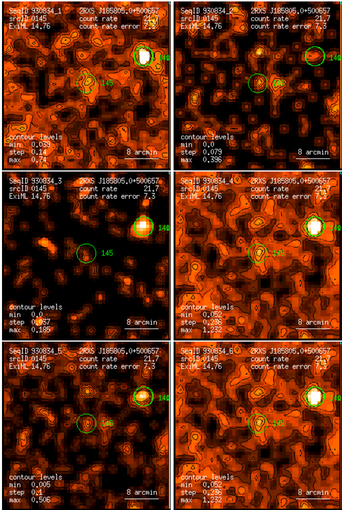
Figure 145: RASS 930834: detection 0145: band rate images, Gaussian filter: (1) PSPC channels 11 – 41, (2) 52 – 90, (3) 91 – 201, (4) 11 – 235, (5) 52 – 201, (6) 11 – 201. Broad band rates in counts/ks. Band rate contour levels in counts/ks/arcmin 2 .
