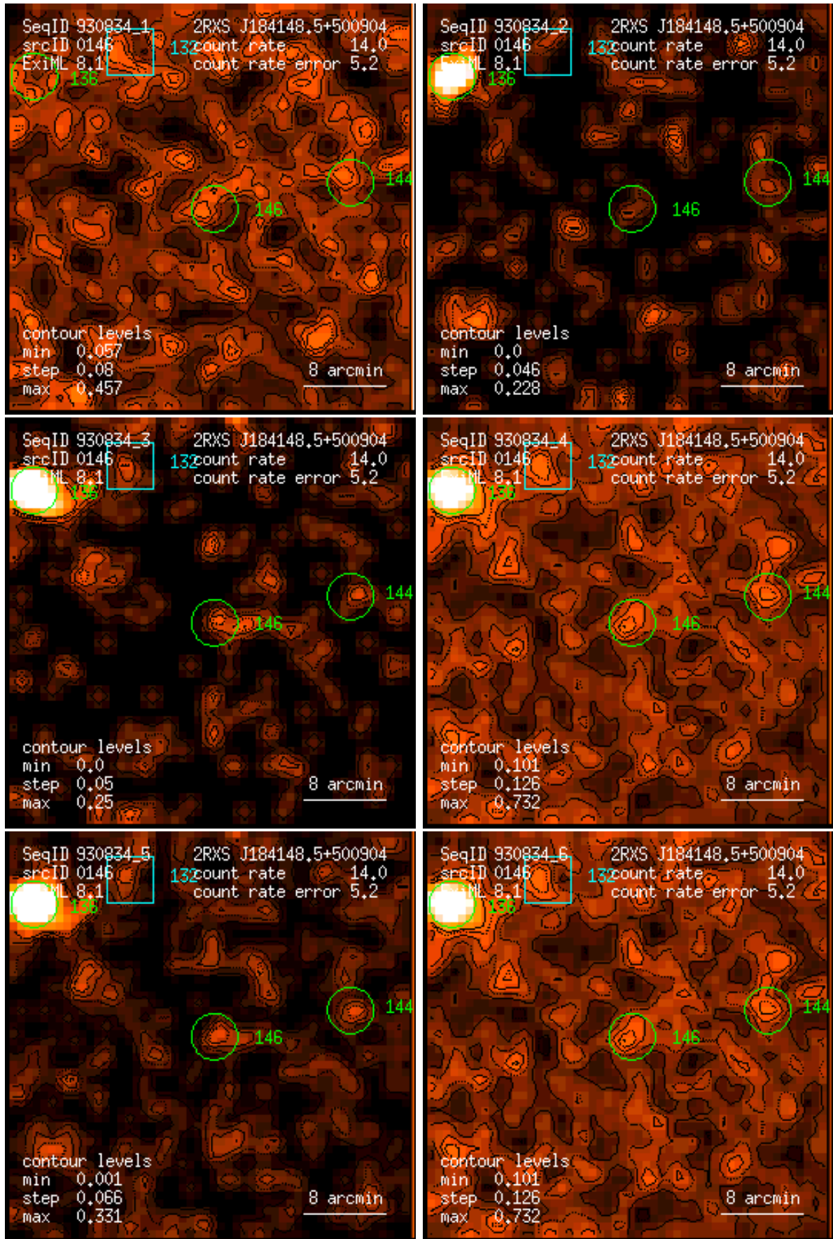
Figure 146: RASS 930834: detection 0146: band rate images, Gaussian filter: (1) PSPC channels 11 – 41, (2) 52 – 90, (3) 91 – 201, (4) 11 – 235, (5) 52 – 201, (6) 11 – 201. Broad band rates in counts/ks. Band rate contour levels in counts/ks/arcmin 2 .
