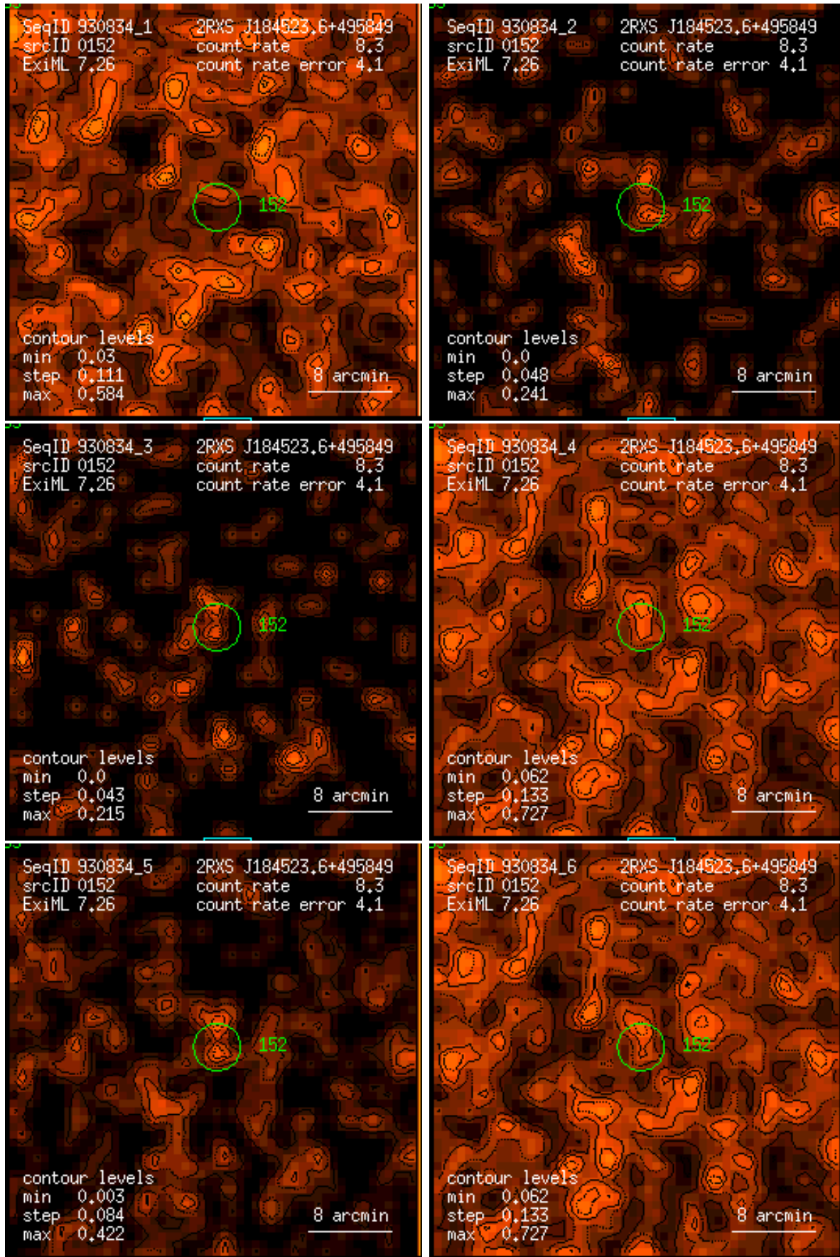
Figure 152: RASS 930834: detection 0152: band rate images, Gaussian filter: (1) PSPC channels 11 – 41, (2) 52 – 90, (3) 91 – 201, (4) 11 – 235, (5) 52 – 201, (6) 11 – 201. Broad band rates in counts/ks. Band rate contour levels in counts/ks/arcmin 2 .
