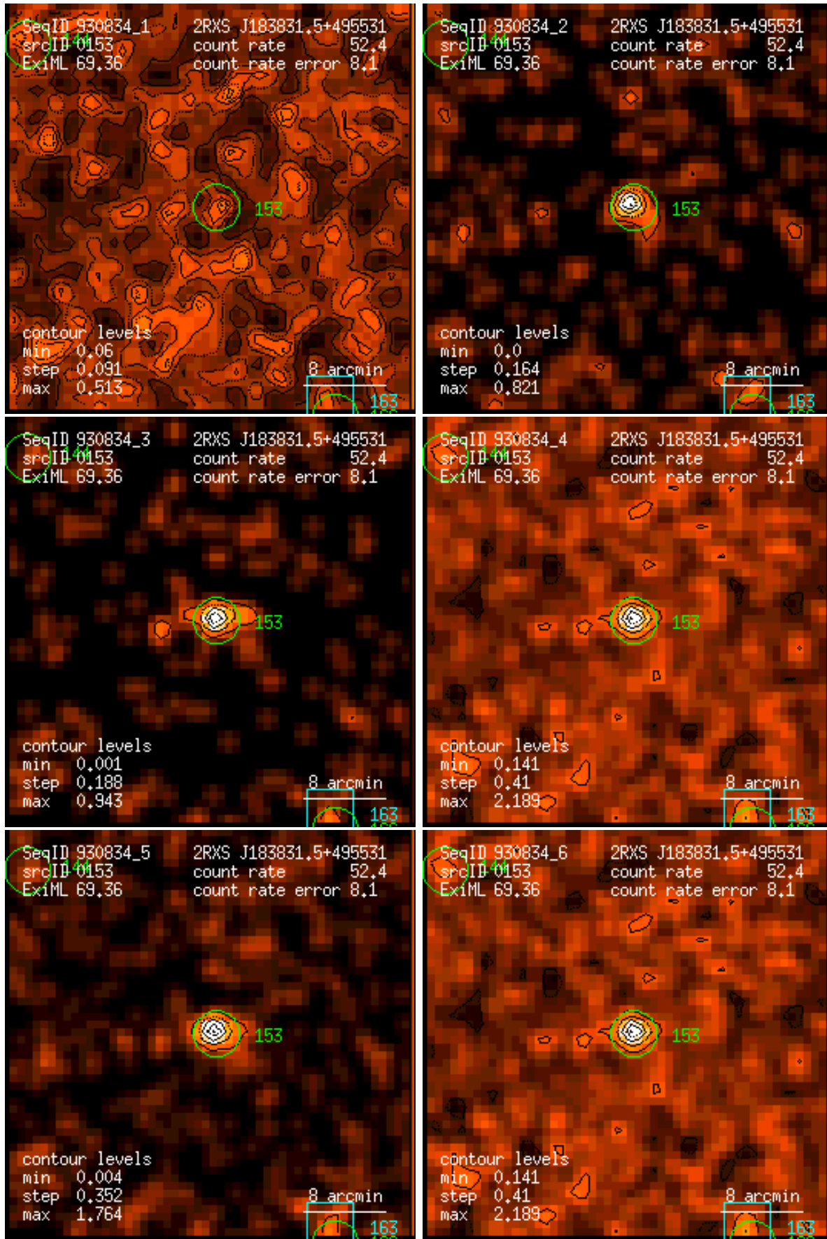
Figure 153: RASS 930834: detection 0153: band rate images, Gaussian filter: (1) PSPC channels 11 – 41, (2) 52 – 90, (3) 91 – 201, (4) 11 – 235, (5) 52 – 201, (6) 11 – 201. Broad band rates in counts/ks. Band rate contour levels in counts/ks/arcmin 2 .
