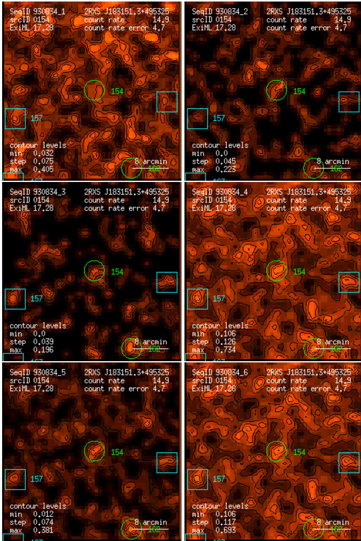
Figure 154: RASS 930834: detection 0154: band rate images, Gaussian filter: (1) PSPC channels 11 – 41, (2) 52 – 90, (3) 91 – 201, (4) 11 – 235, (5) 52 – 201, (6) 11 – 201. Broad band rates in counts/ks. Band rate contour levels in counts/ks/arcmin 2 .
