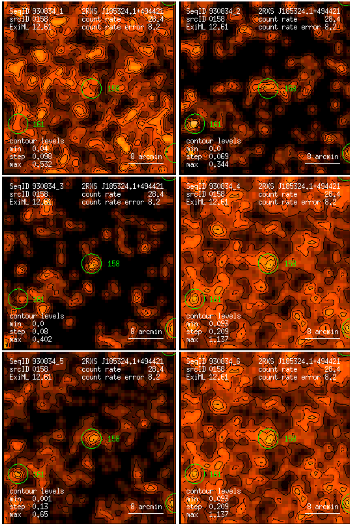
Figure 158: RASS 930834: detection 0158: band rate images, Gaussian filter: (1) PSPC channels 11 – 41, (2) 52 – 90, (3) 91 – 201, (4) 11 – 235, (5) 52 – 201, (6) 11 – 201. Broad band rates in counts/ks. Band rate contour levels in counts/ks/arcmin 2 .
