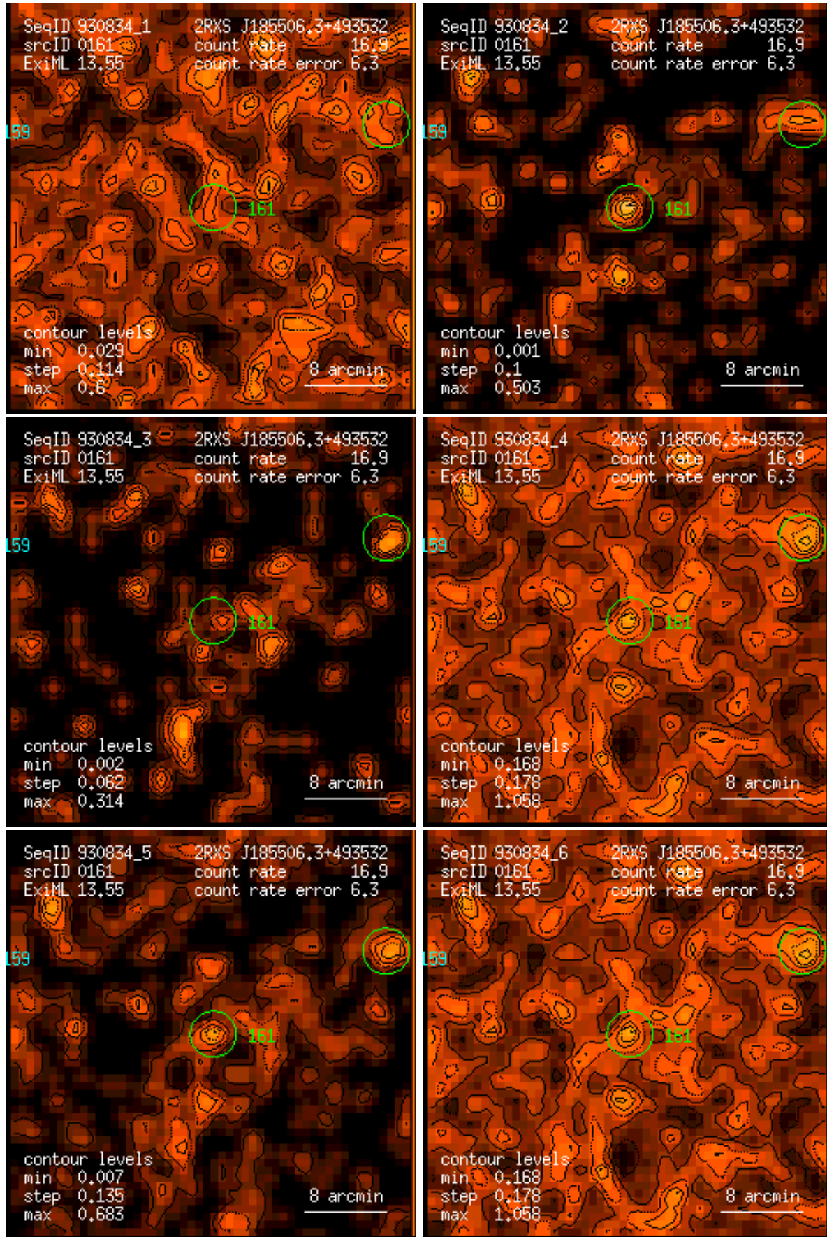
Figure 161: RASS 930834: detection 0161: band rate images, Gaussian filter: (1) PSPC channels 11 – 41, (2) 52 – 90, (3) 91 – 201, (4) 11 – 235, (5) 52 – 201, (6) 11 – 201. Broad band rates in counts/ks. Band rate contour levels in counts/ks/arcmin 2 .
