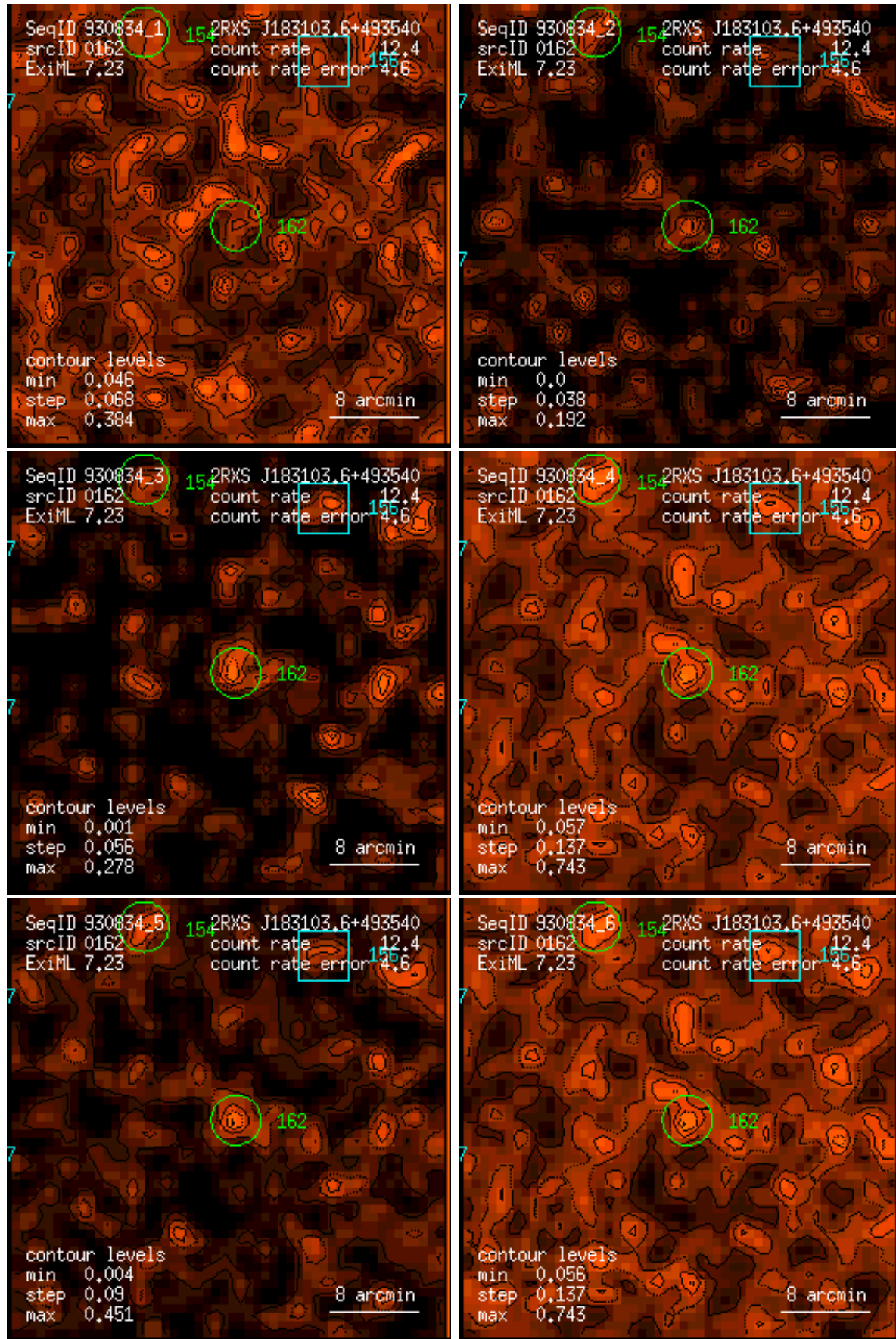
Figure 162: RASS 930834: detection 0162: band rate images, Gaussian filter: (1) PSPC channels 11 – 41, (2) 52 – 90, (3) 91 – 201, (4) 11 – 235, (5) 52 – 201, (6) 11 – 201. Broad band rates in counts/ks. Band rate contour levels in counts/ks/arcmin 2 .
