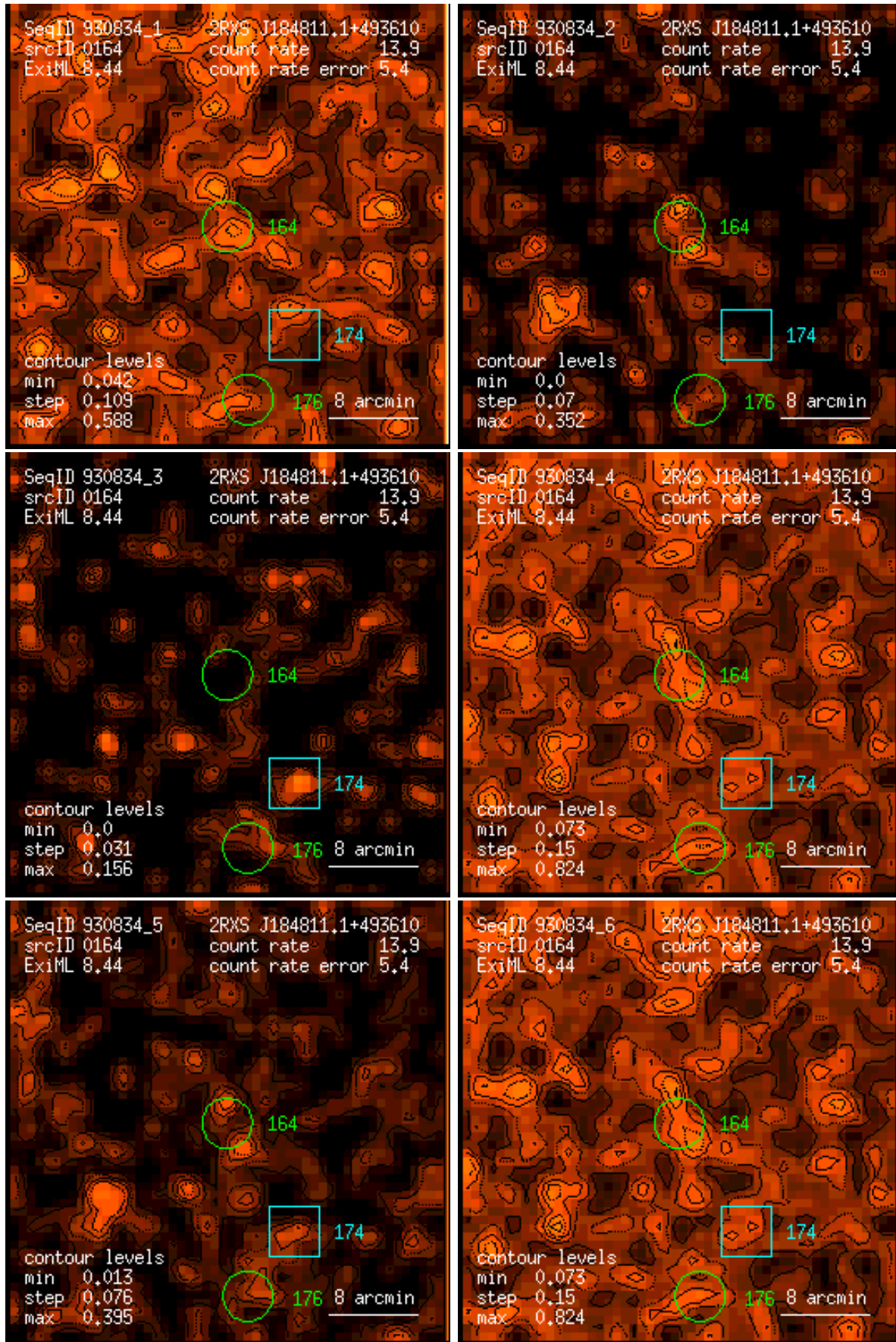
Figure 164: RASS 930834: detection 0164: band rate images, Gaussian filter: (1) PSPC channels 11 – 41, (2) 52 – 90, (3) 91 – 201, (4) 11 – 235, (5) 52 – 201, (6) 11 – 201. Broad band rates in counts/ks. Band rate contour levels in counts/ks/arcmin 2 .
