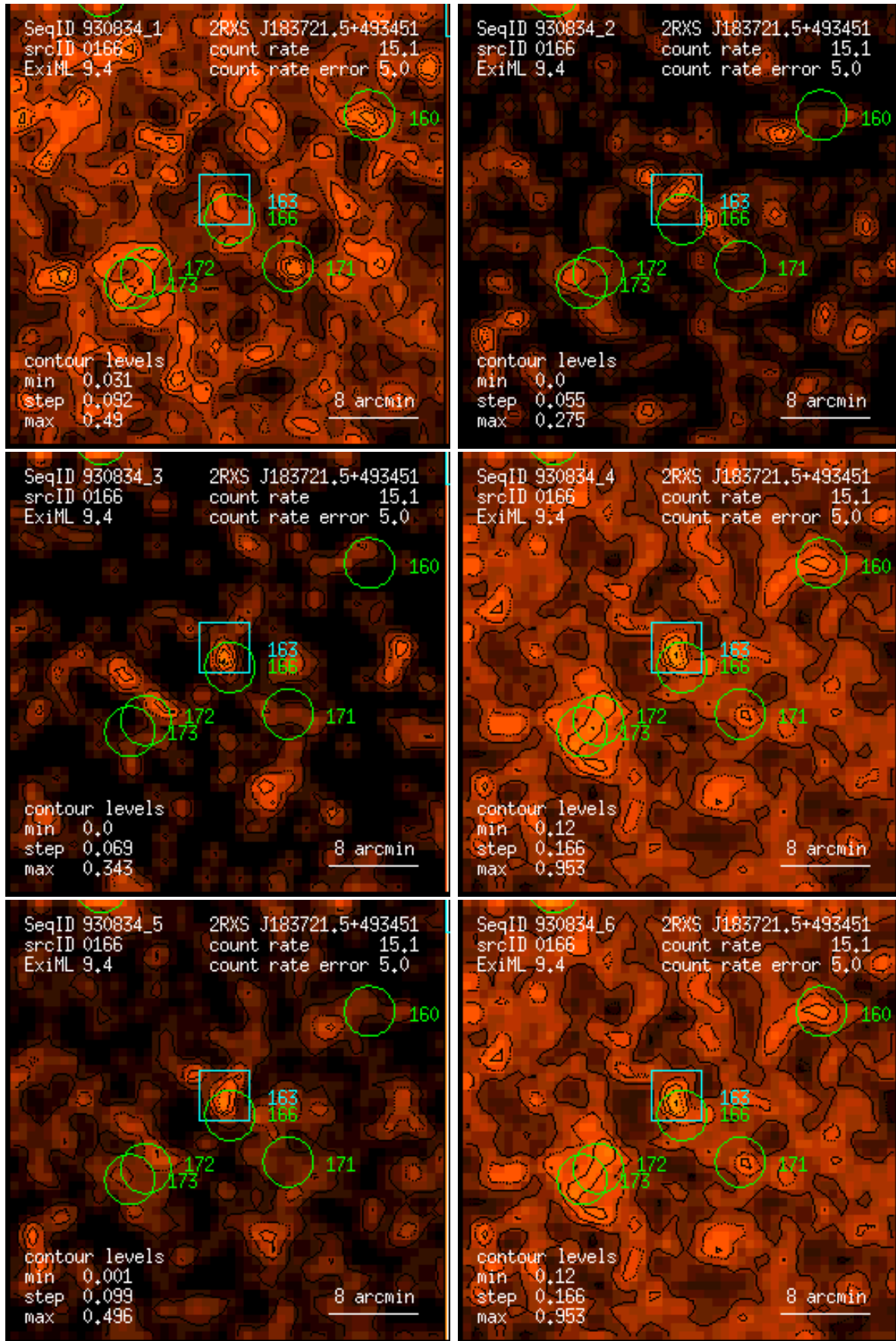
Figure 166: RASS 930834: detection 0166: band rate images, Gaussian filter: (1) PSPC channels 11 – 41, (2) 52 – 90, (3) 91 – 201, (4) 11 – 235, (5) 52 – 201, (6) 11 – 201. Broad band rates in counts/ks. Band rate contour levels in counts/ks/arcmin 2 .
