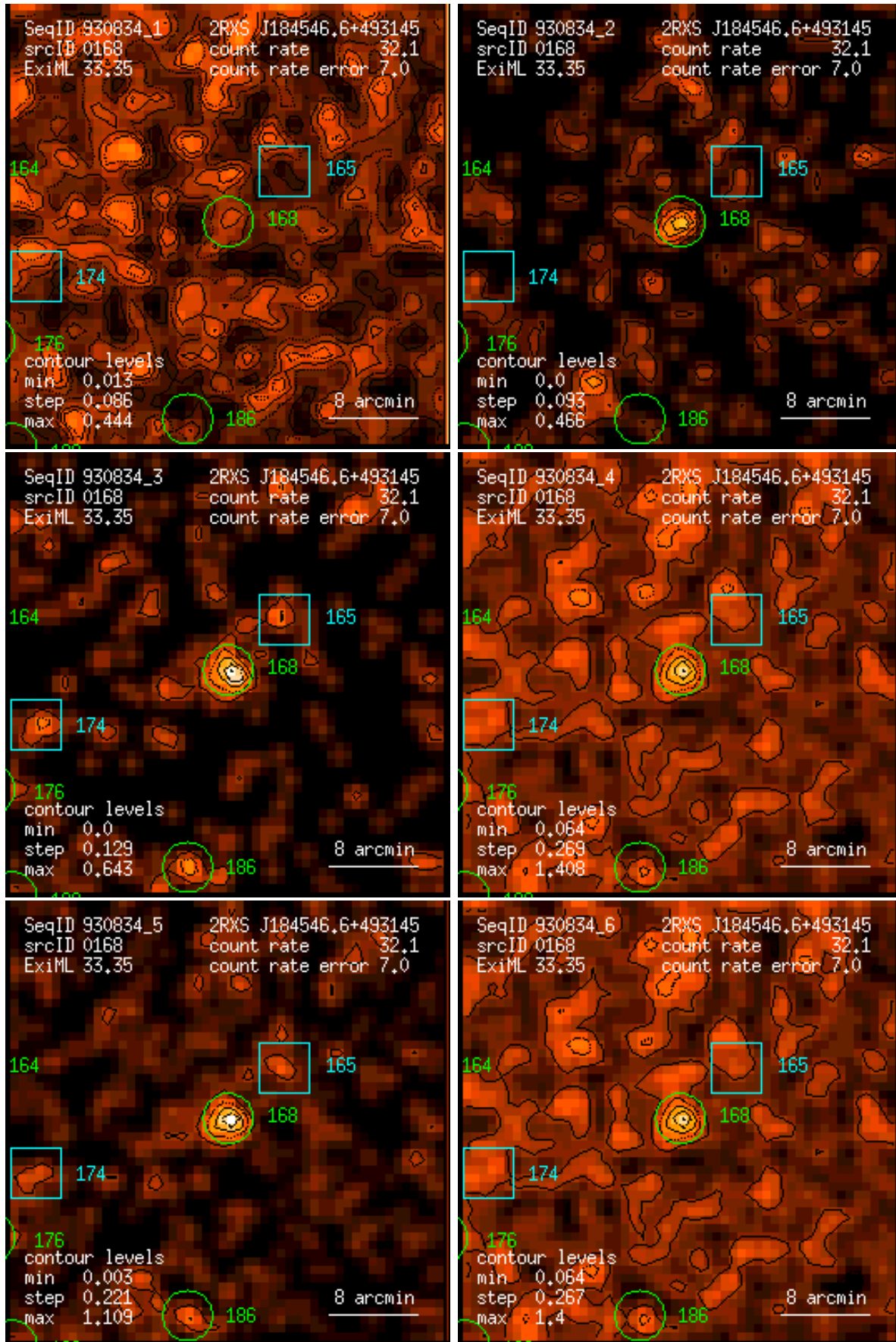
Figure 168: RASS 930834: detection 0168: band rate images, Gaussian filter: (1) PSPC channels 11 – 41, (2) 52 – 90, (3) 91 – 201, (4) 11 – 235, (5) 52 – 201, (6) 11 – 201. Broad band rates in counts/ks. Band rate contour levels in counts/ks/arcmin 2 .
