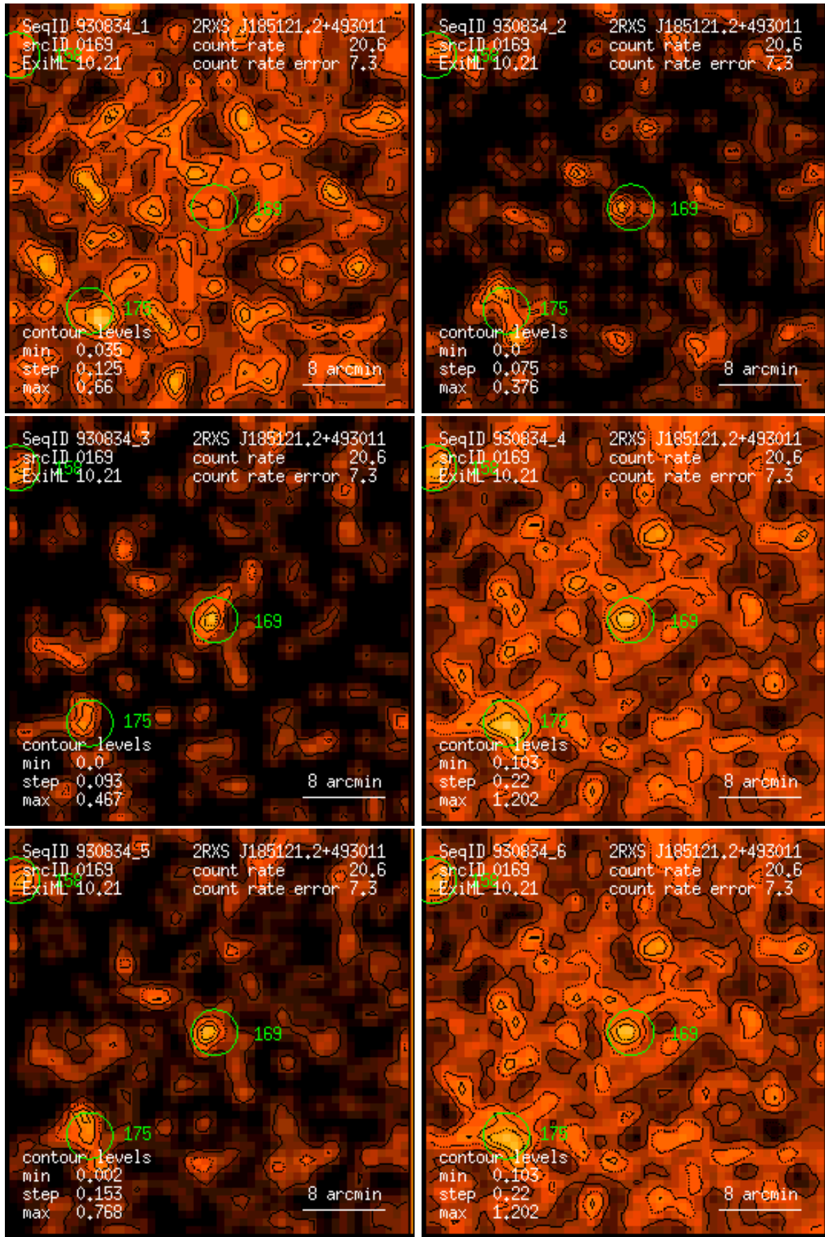
Figure 169: RASS 930834: detection 0169: band rate images, Gaussian filter: (1) PSPC channels 11 – 41, (2) 52 – 90, (3) 91 – 201, (4) 11 – 235, (5) 52 – 201, (6) 11 – 201. Broad band rates in counts/ks. Band rate contour levels in counts/ks/arcmin 2 .
