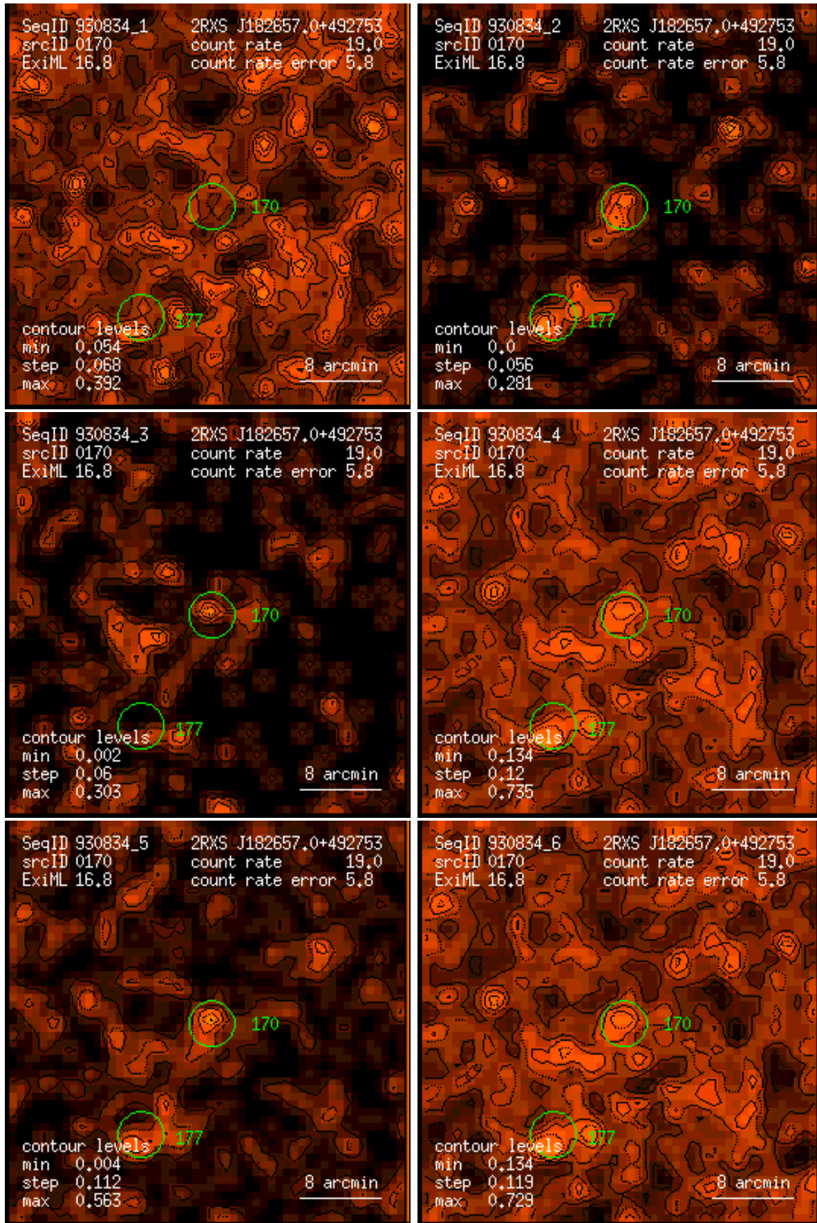
Figure 170: RASS 930834: detection 0170: band rate images, Gaussian filter: (1) PSPC channels 11 – 41, (2) 52 – 90, (3) 91 – 201, (4) 11 – 235, (5) 52 – 201, (6) 11 – 201. Broad band rates in counts/ks. Band rate contour levels in counts/ks/arcmin 2 .
